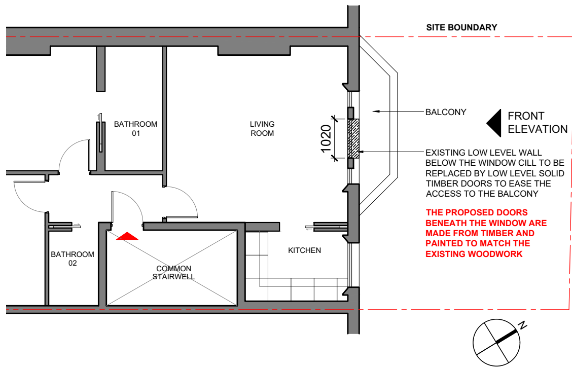
1 EXISTING FIRST FLOOR PLAN_ SCALE 1:100 @ A3
