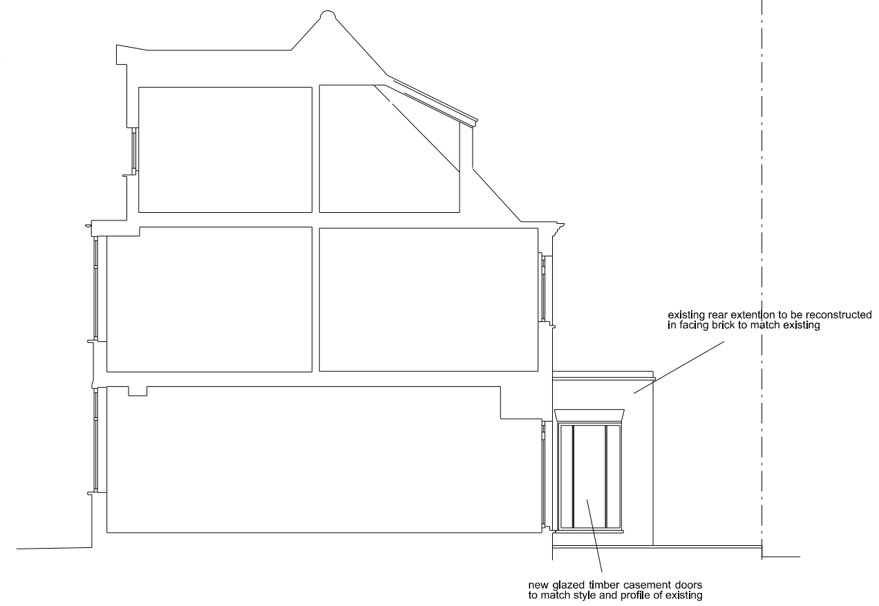
Datum: 78.00m. Section 1. Proposed Side Section Elevation
