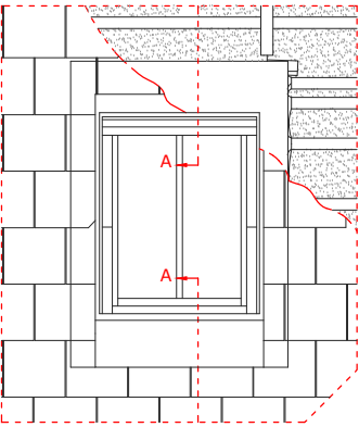
Typical Elevation
