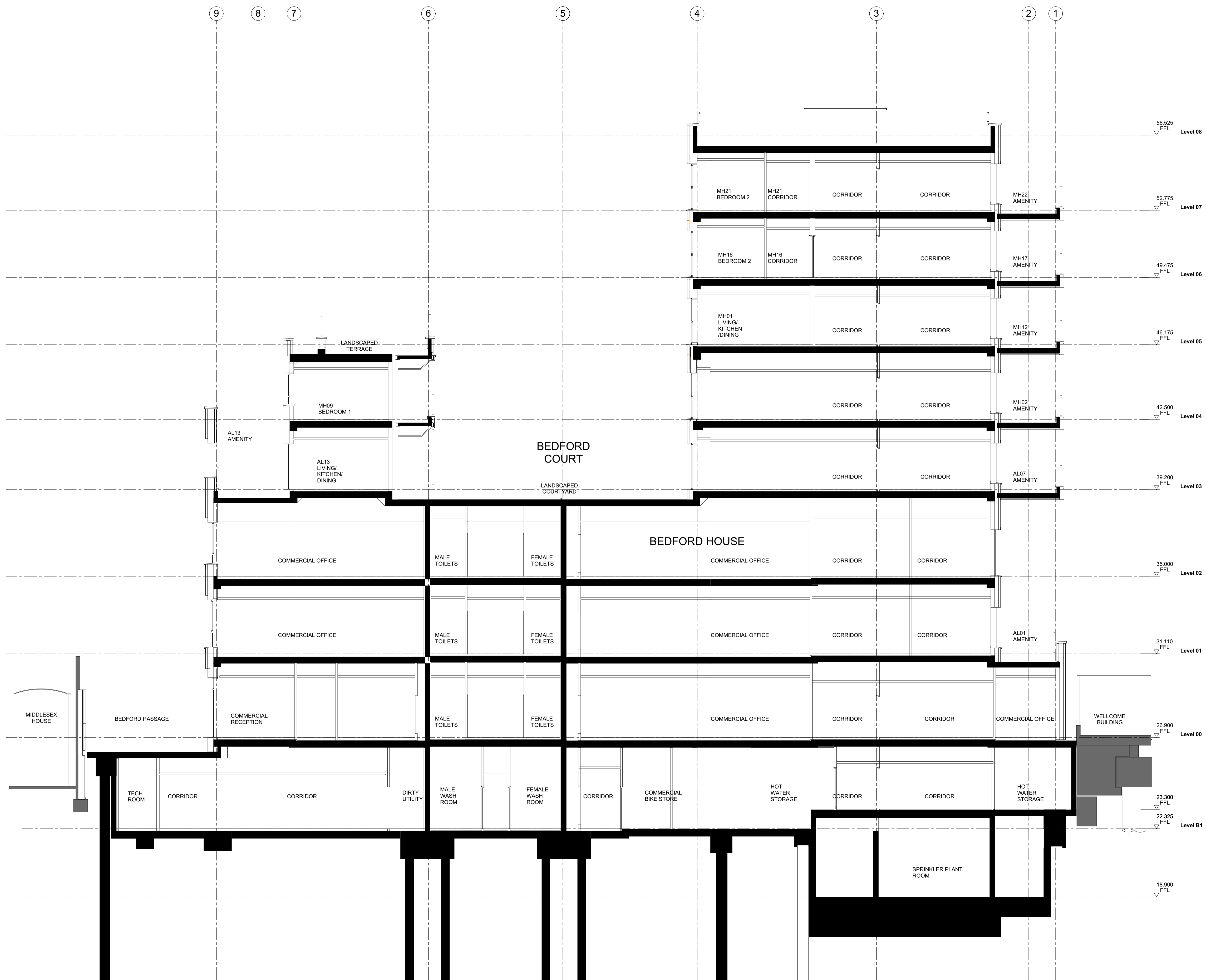
SECTION BB
