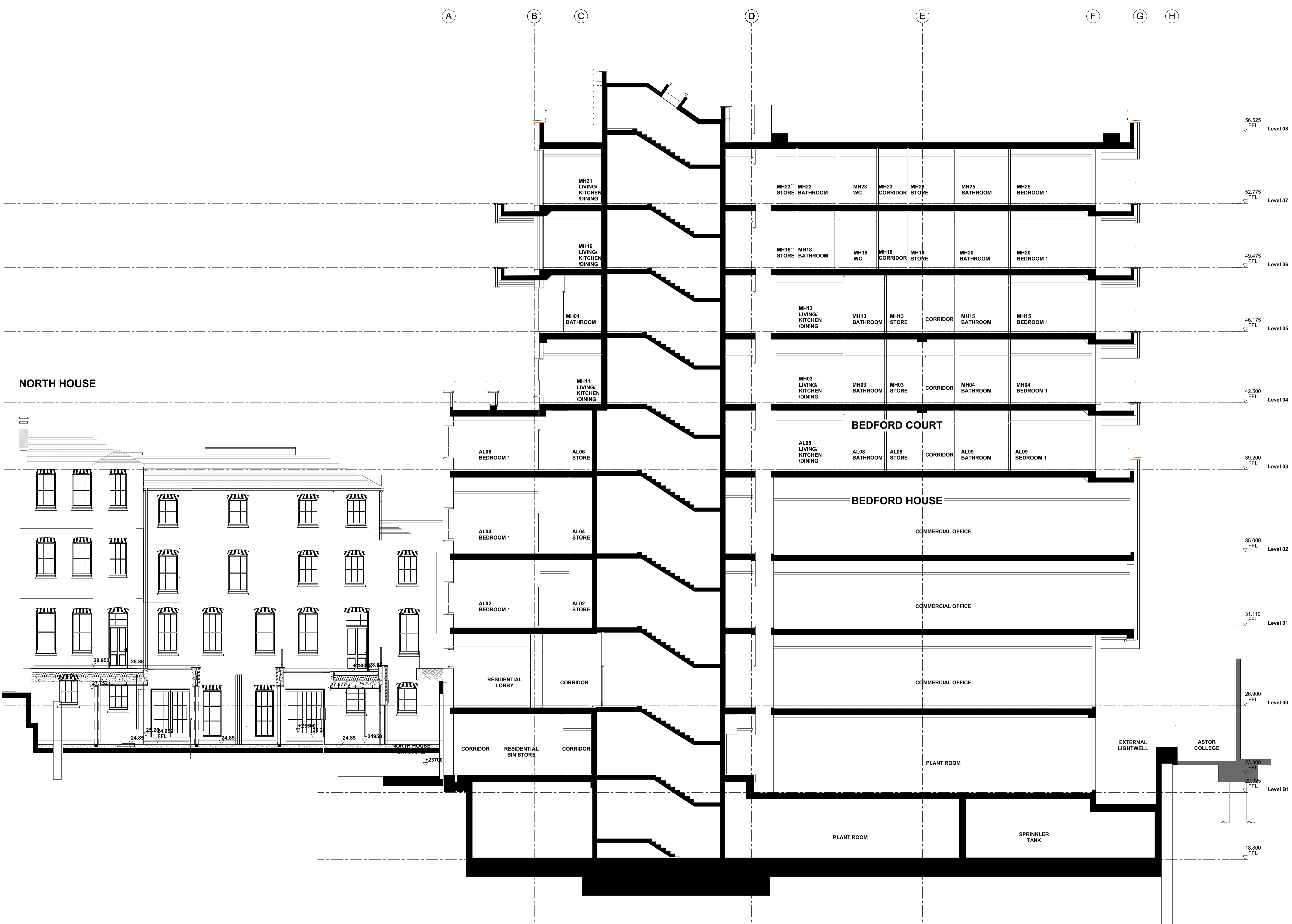
SECTION AA
