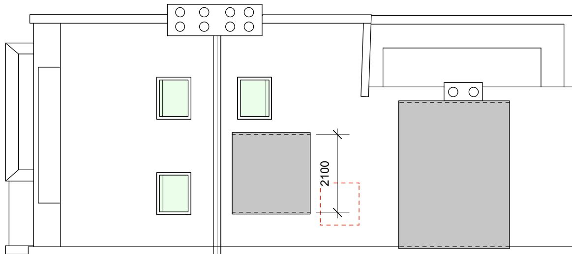
Roof Plan
