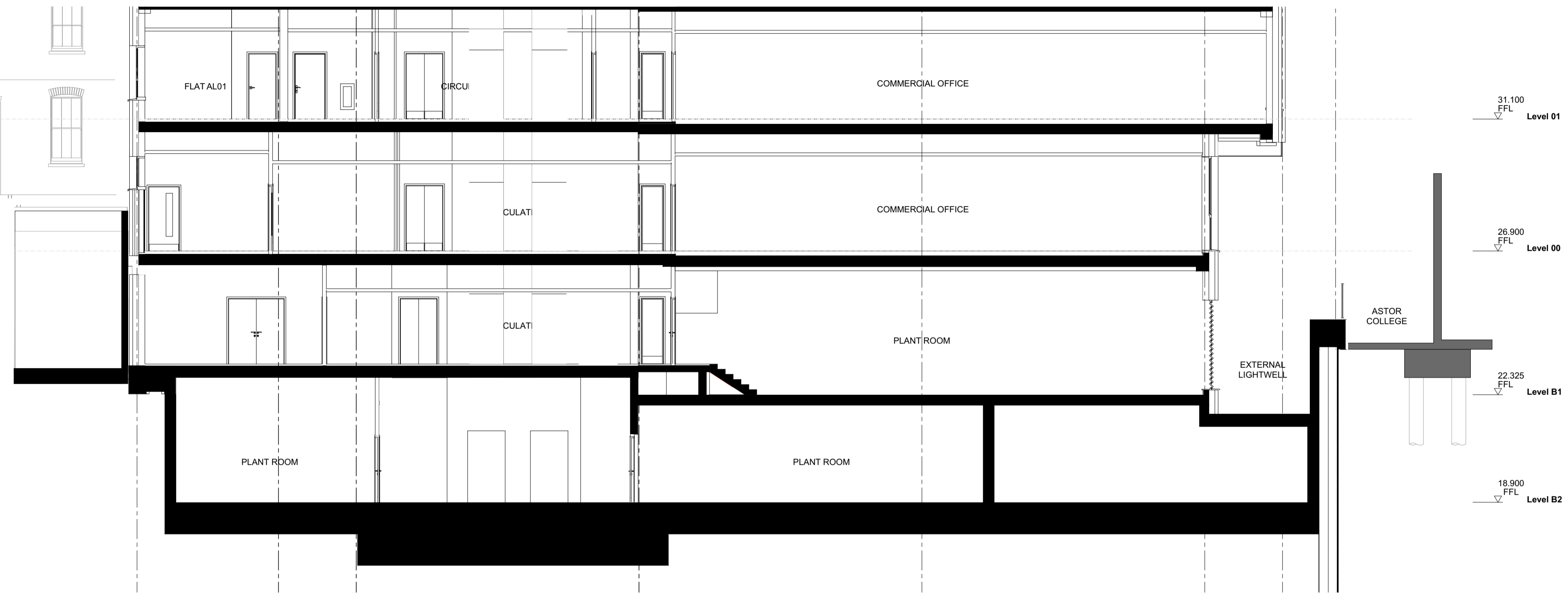
SECTION GG
