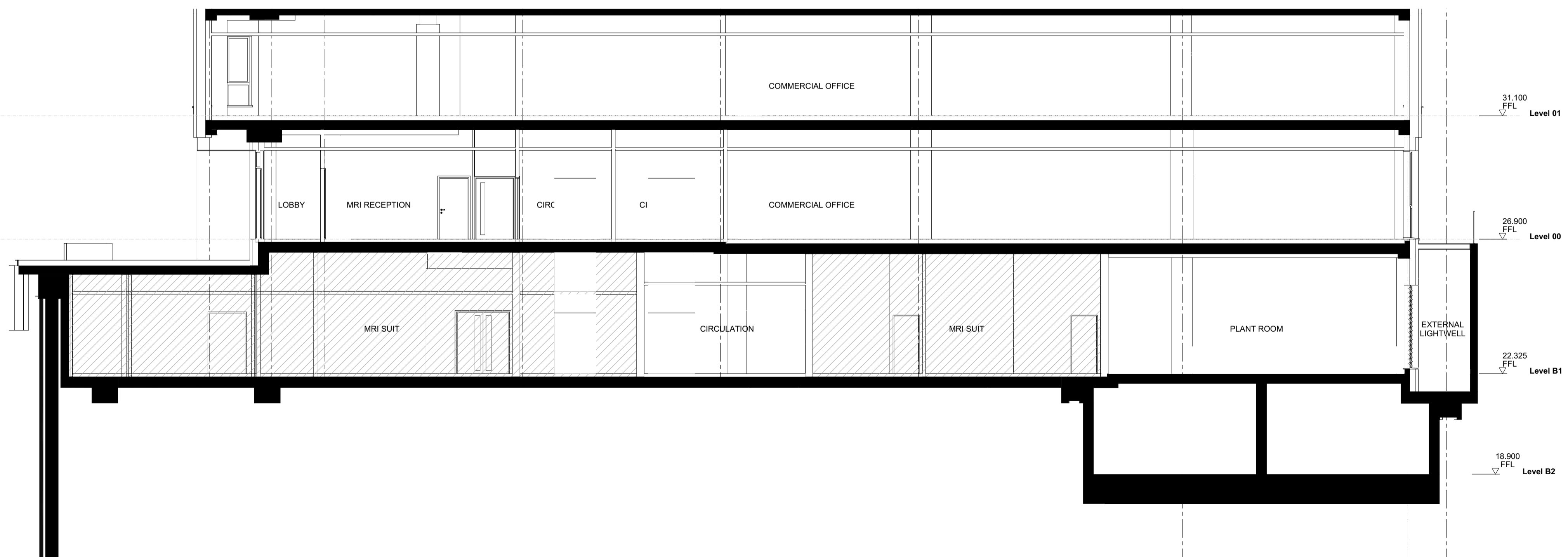
SECTION HH
