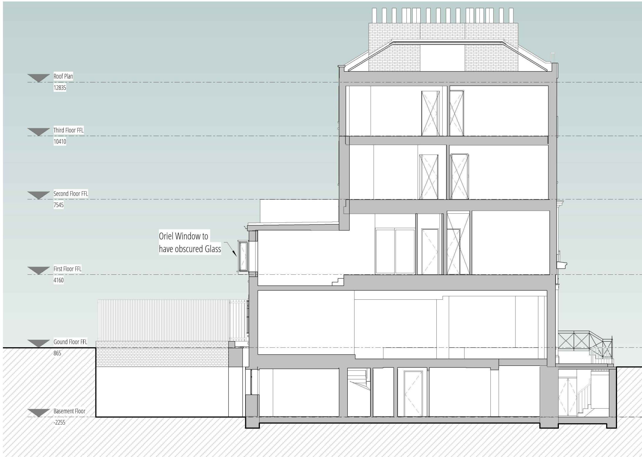
1 Proposed Section BB' 1: 100
