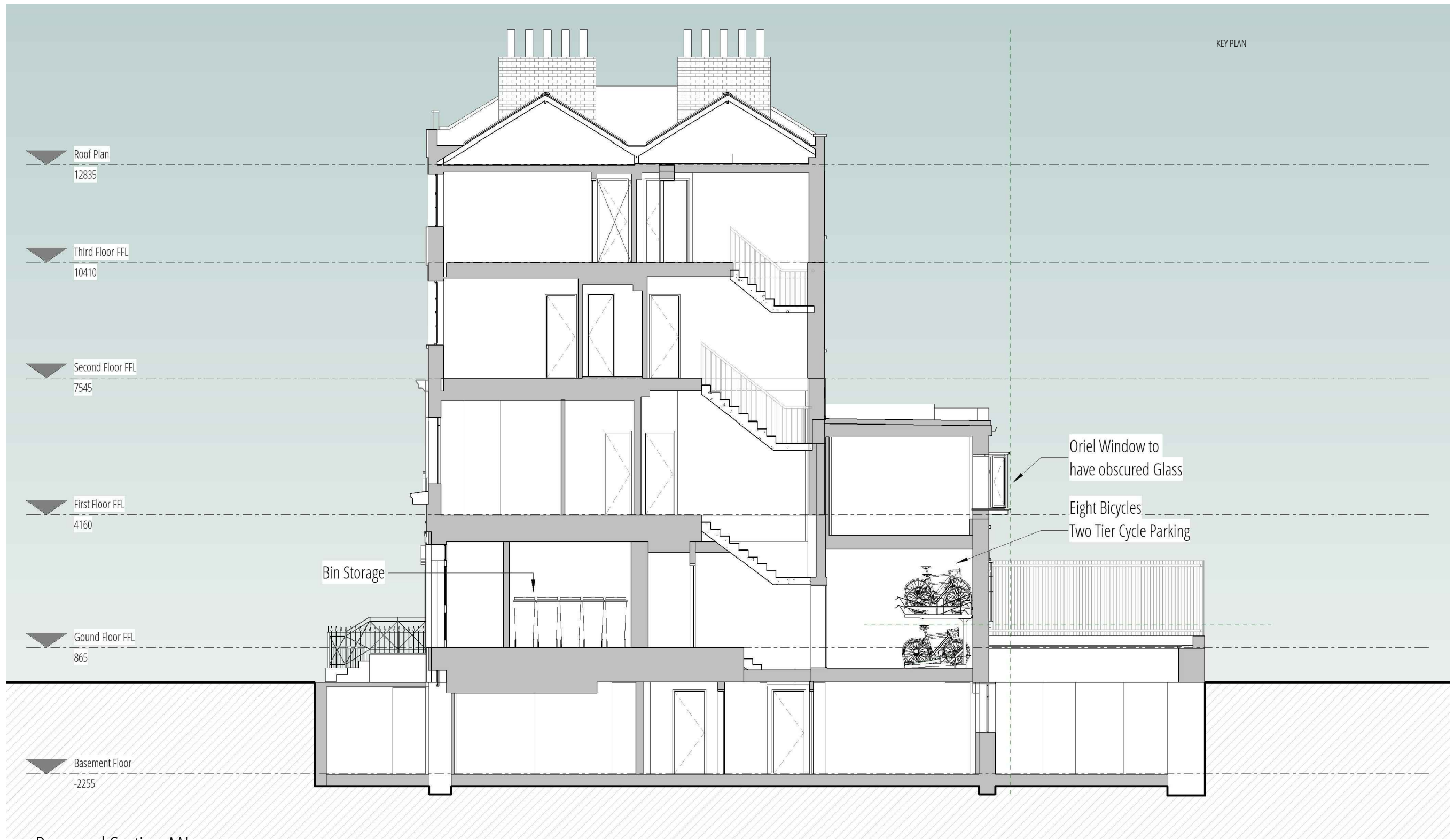
1 Proposed Section AA' 1:100
