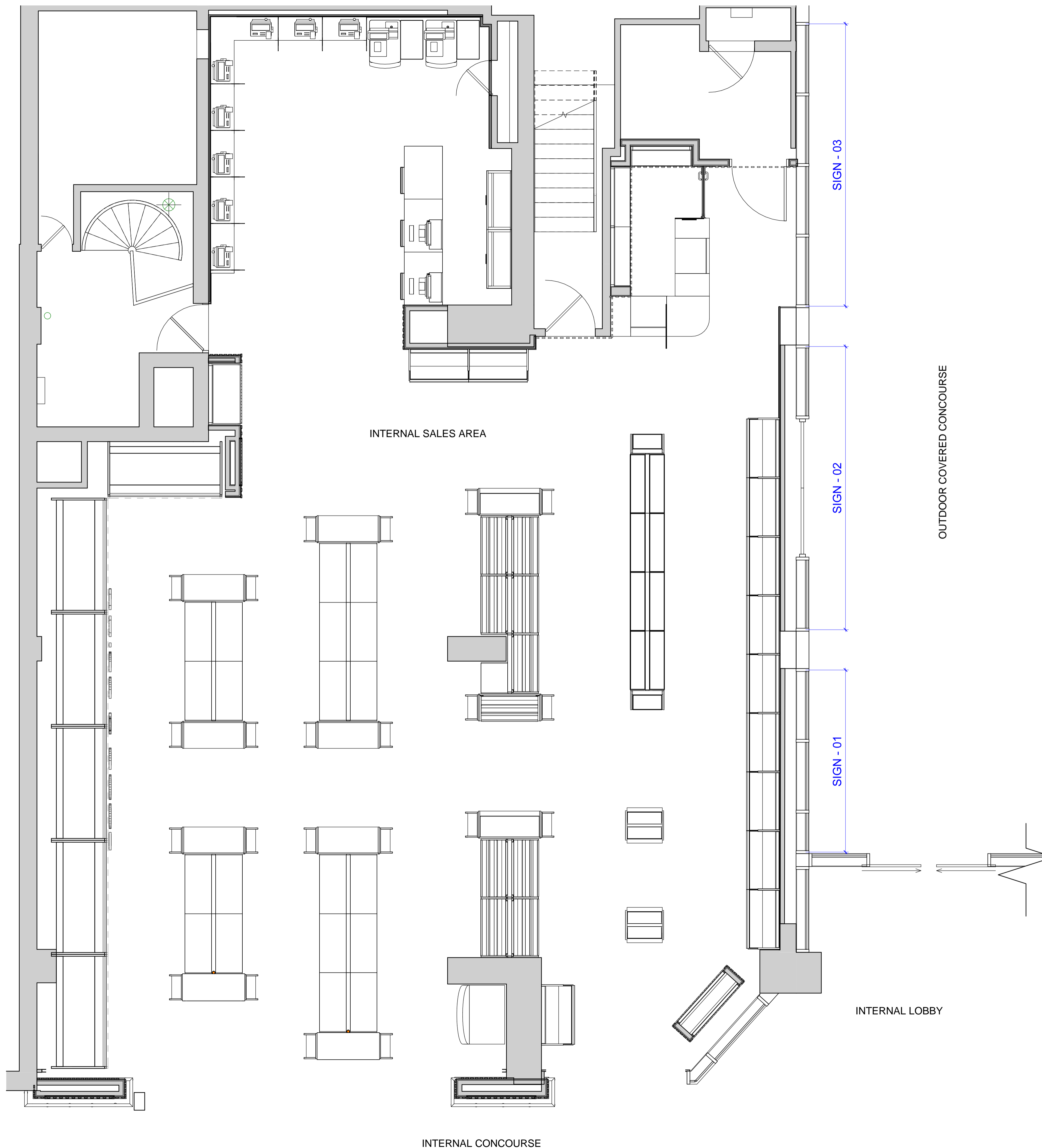
1 PROPOSED GROUND FLOOR GA PLAN 1 : 35
