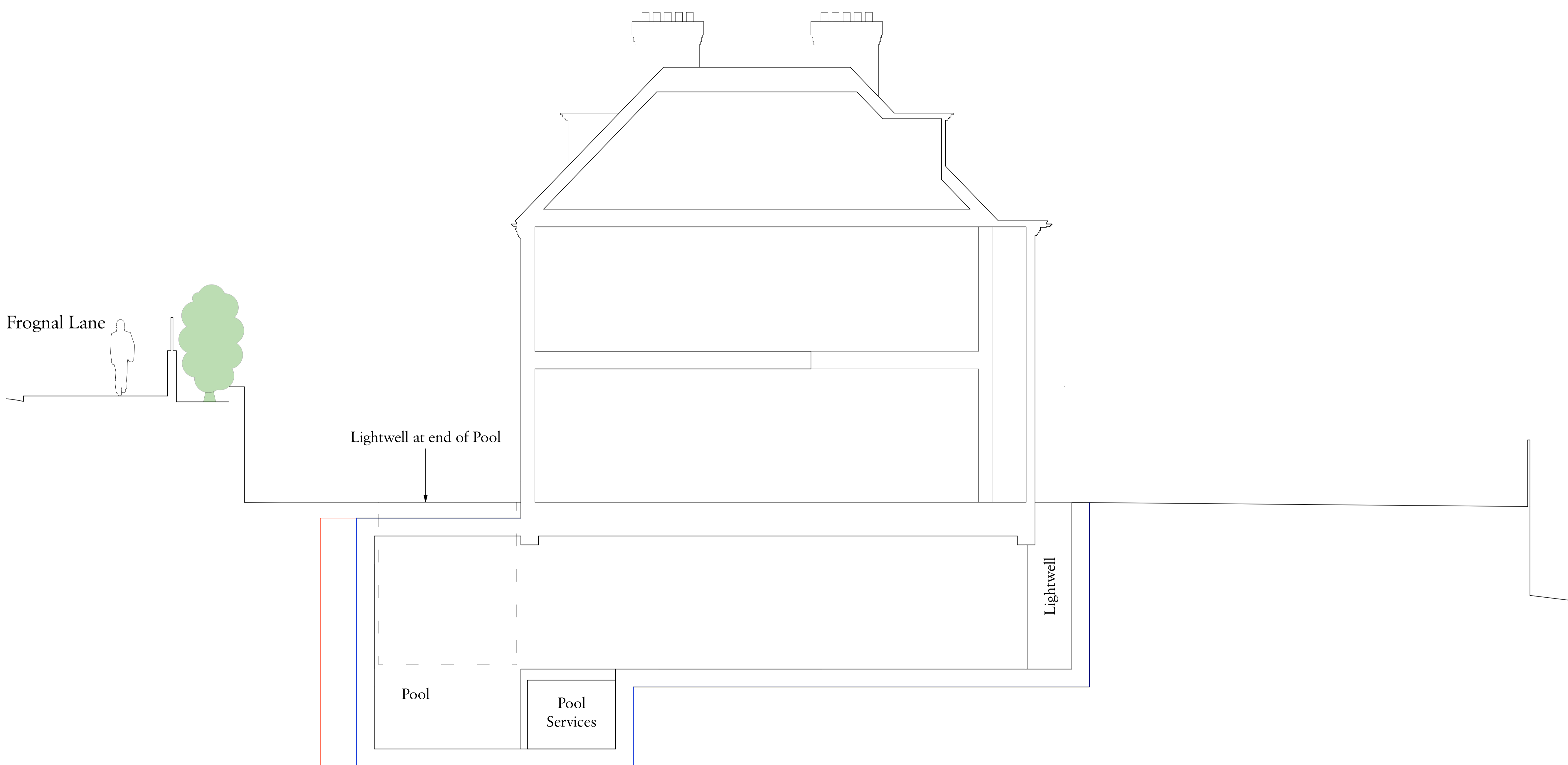
1 Proposed Section - BB Scale: 1:50
