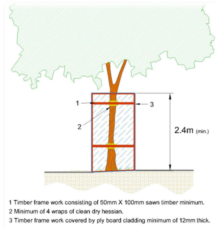
Figure 4: Example image of Protective barrier hoarding
