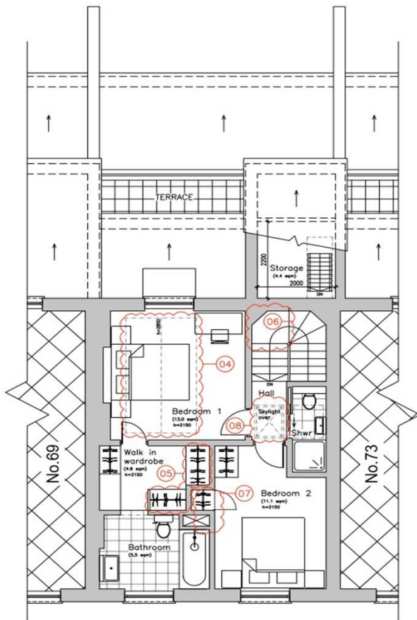
Surveyed Third floor plan
