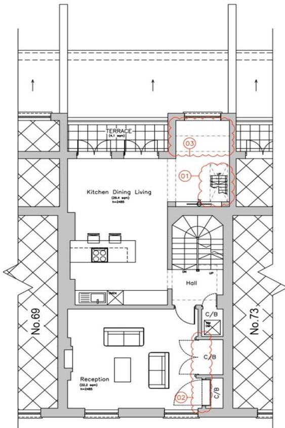
Surveyed Second floor plan
