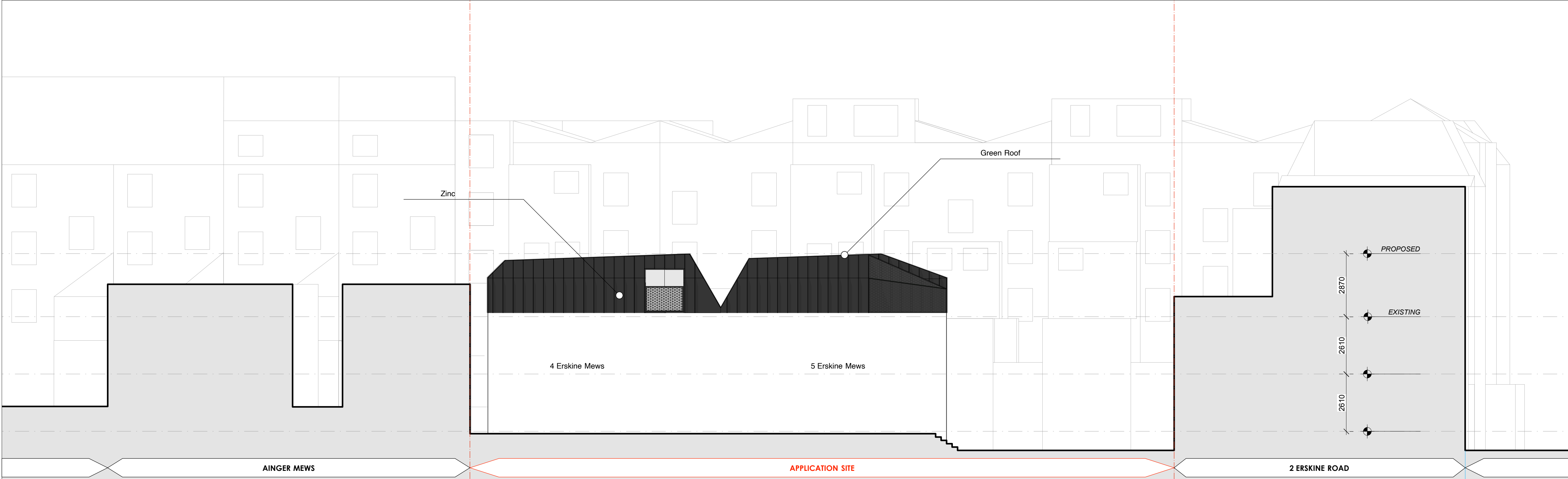
01 Proposed Mews Elevation West GE.03 1:100 @ A1 | 1:200 @ A3
