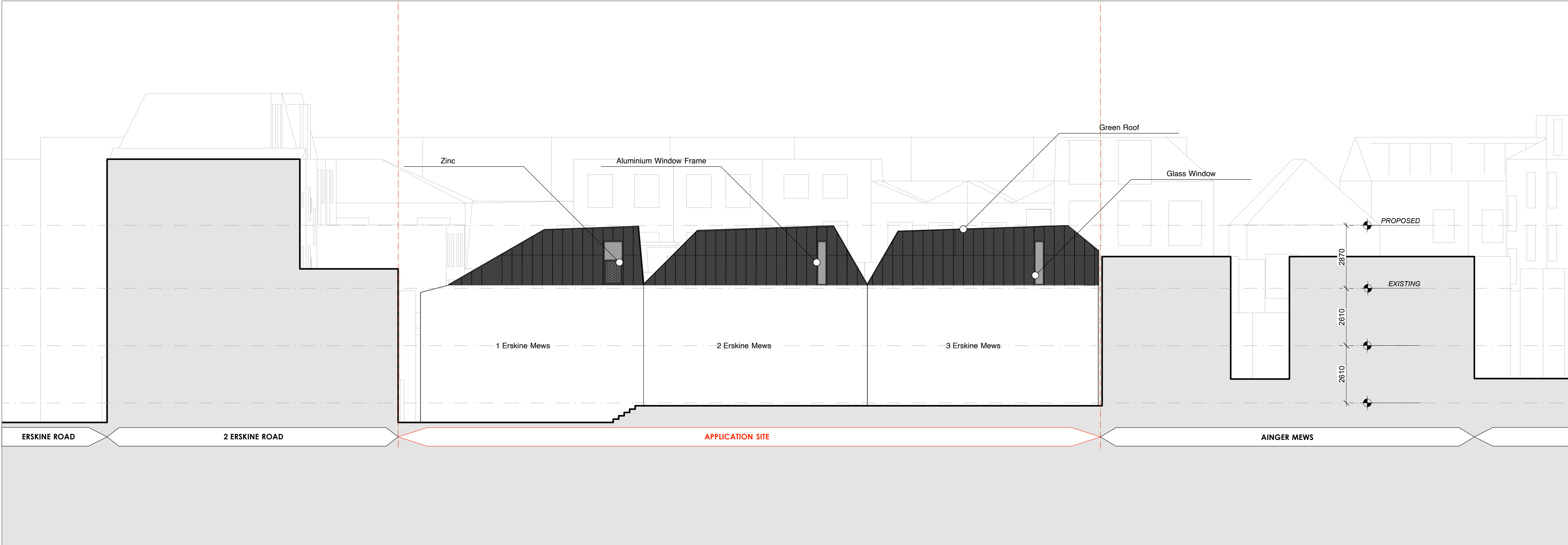
01 Proposed Mews Elevation West GE.03 1:100 @ A1 | 1:200 @ A3
