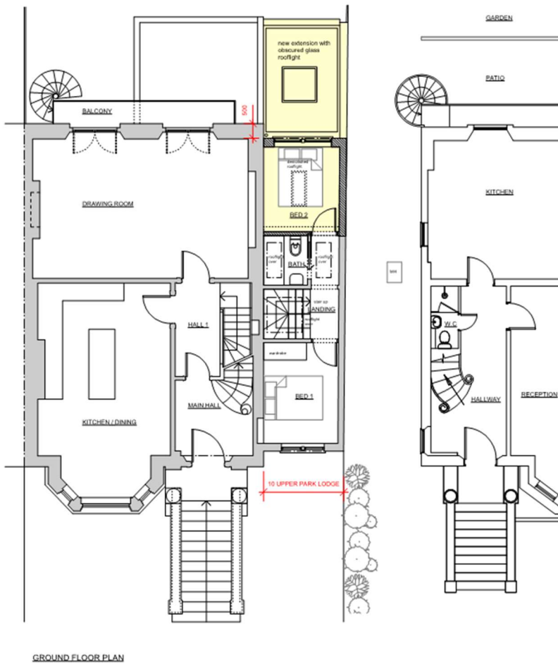
Image 6 Ground Floor Plan
