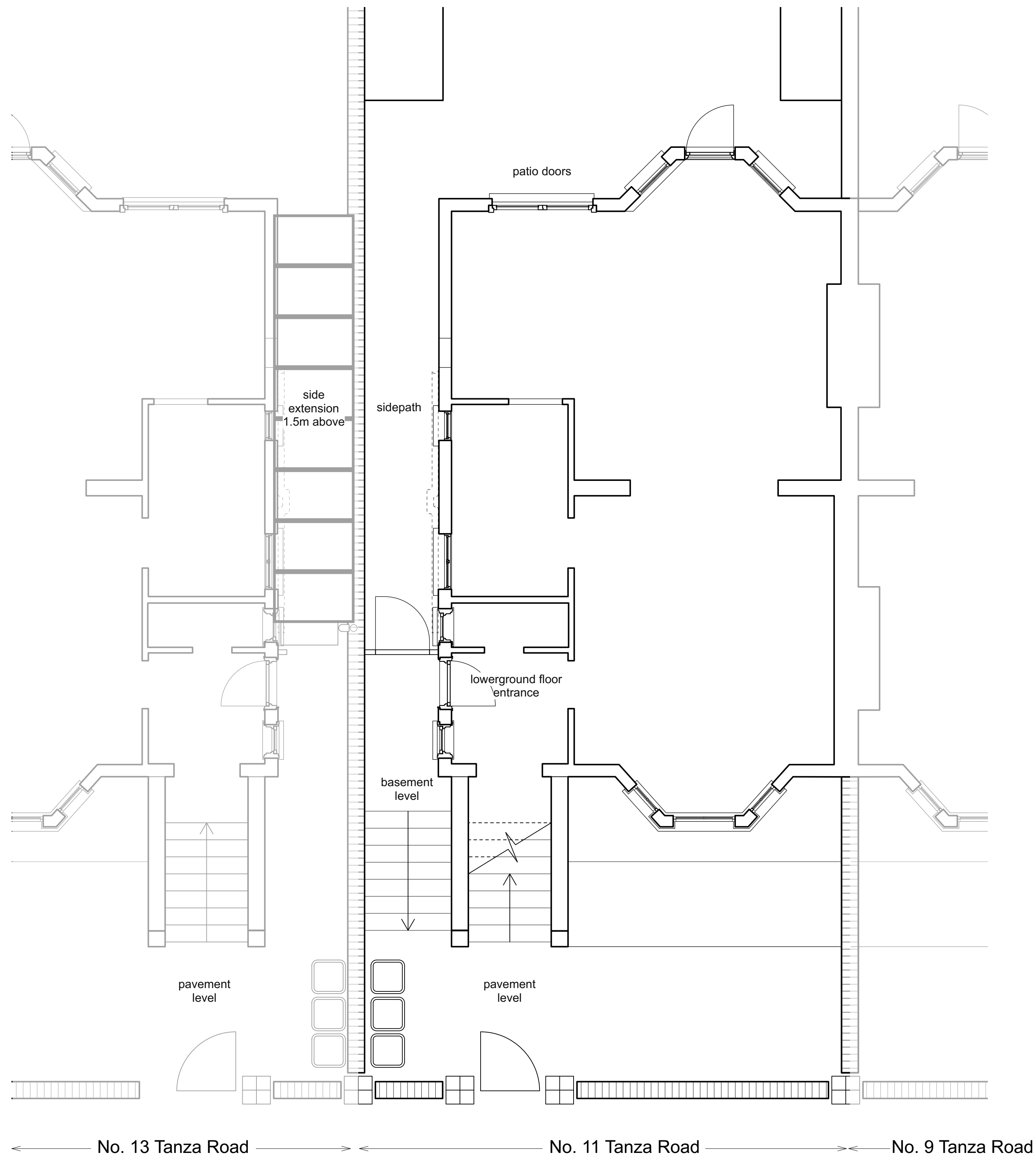
1 Existing Lower Ground Floor Plan Scale: 1/100
