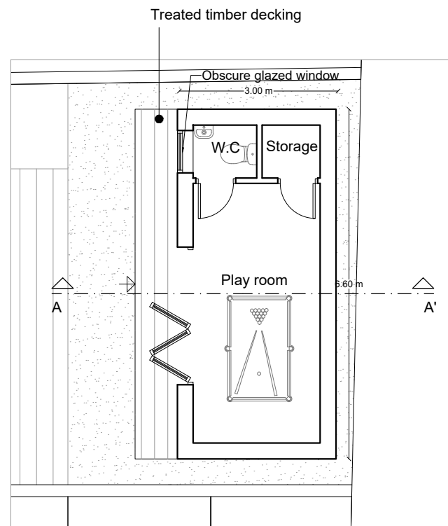
Floor Plan
