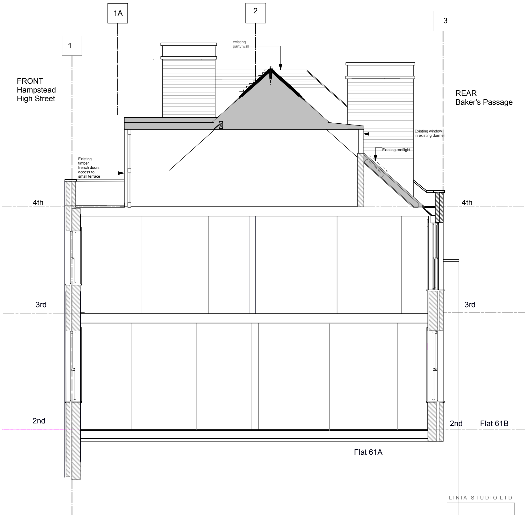
Existing Section taken through existing dormers
