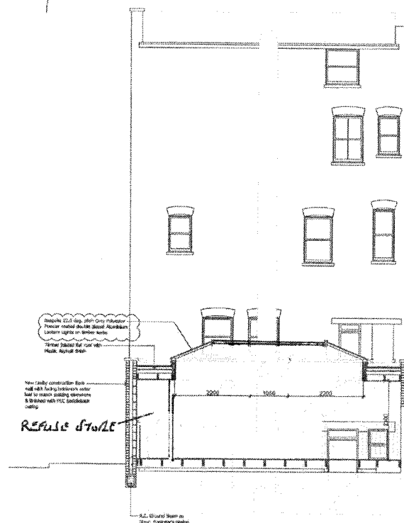
Part Flank Elevation to Inglewood Rd As Proposed
