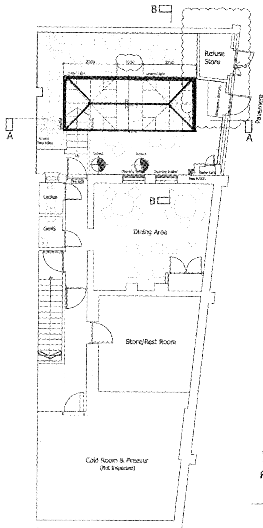
Lower Ground Floor Plan (Ground Floor Unaffected)
