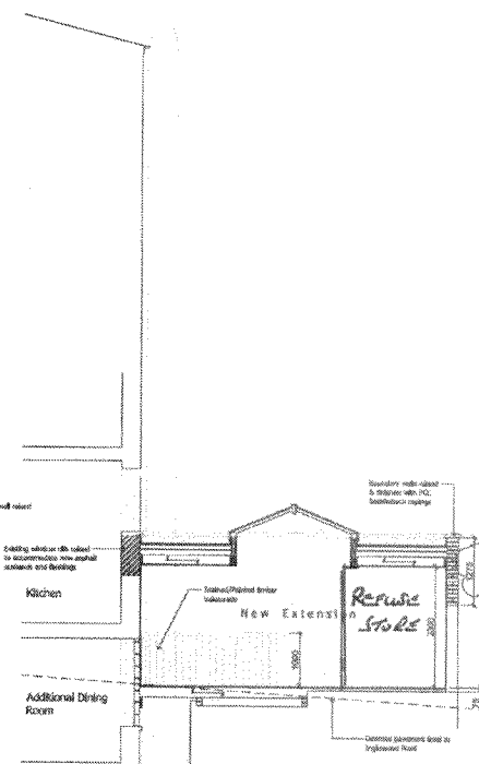
Part Flank Elevation to Inglewood Rd As Proposed
