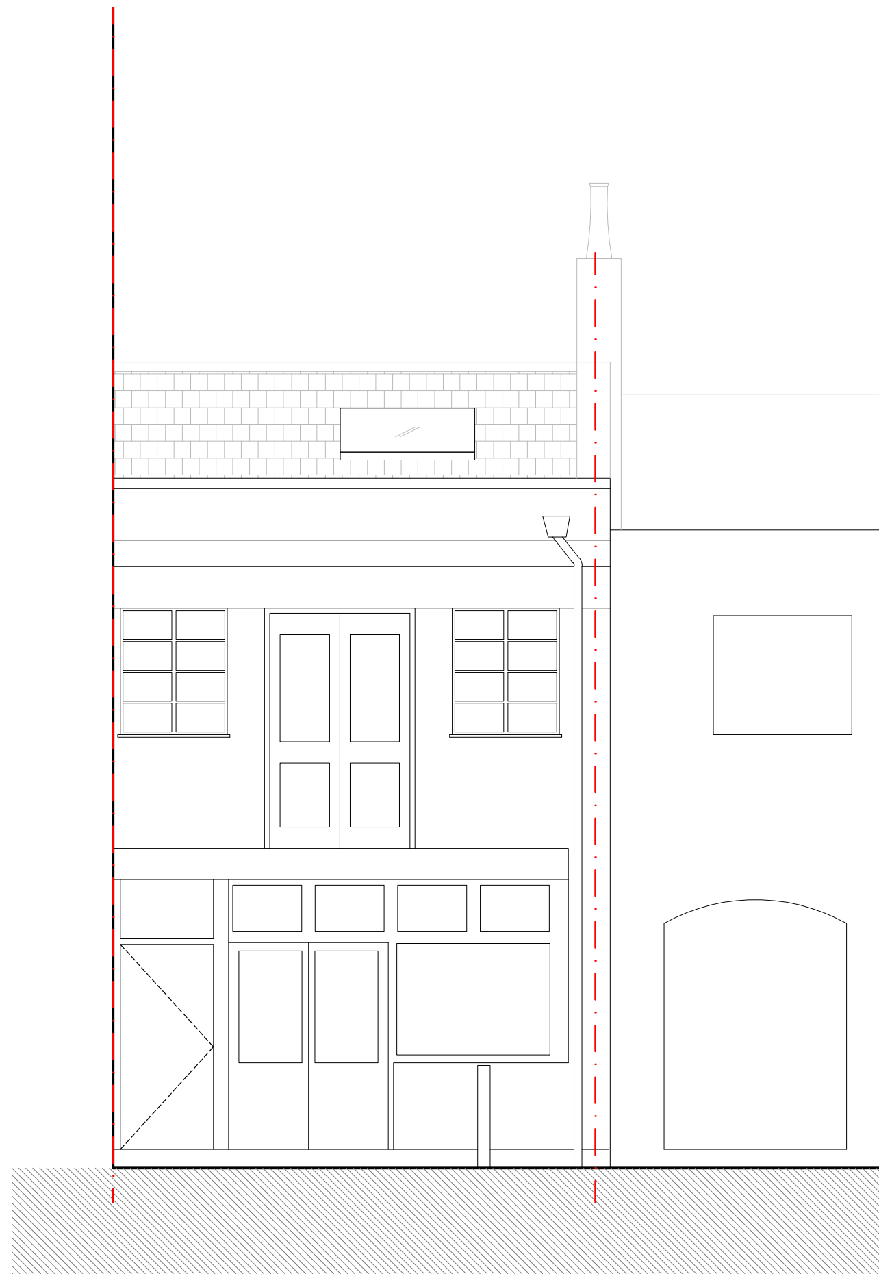
WEST ELEVATION
