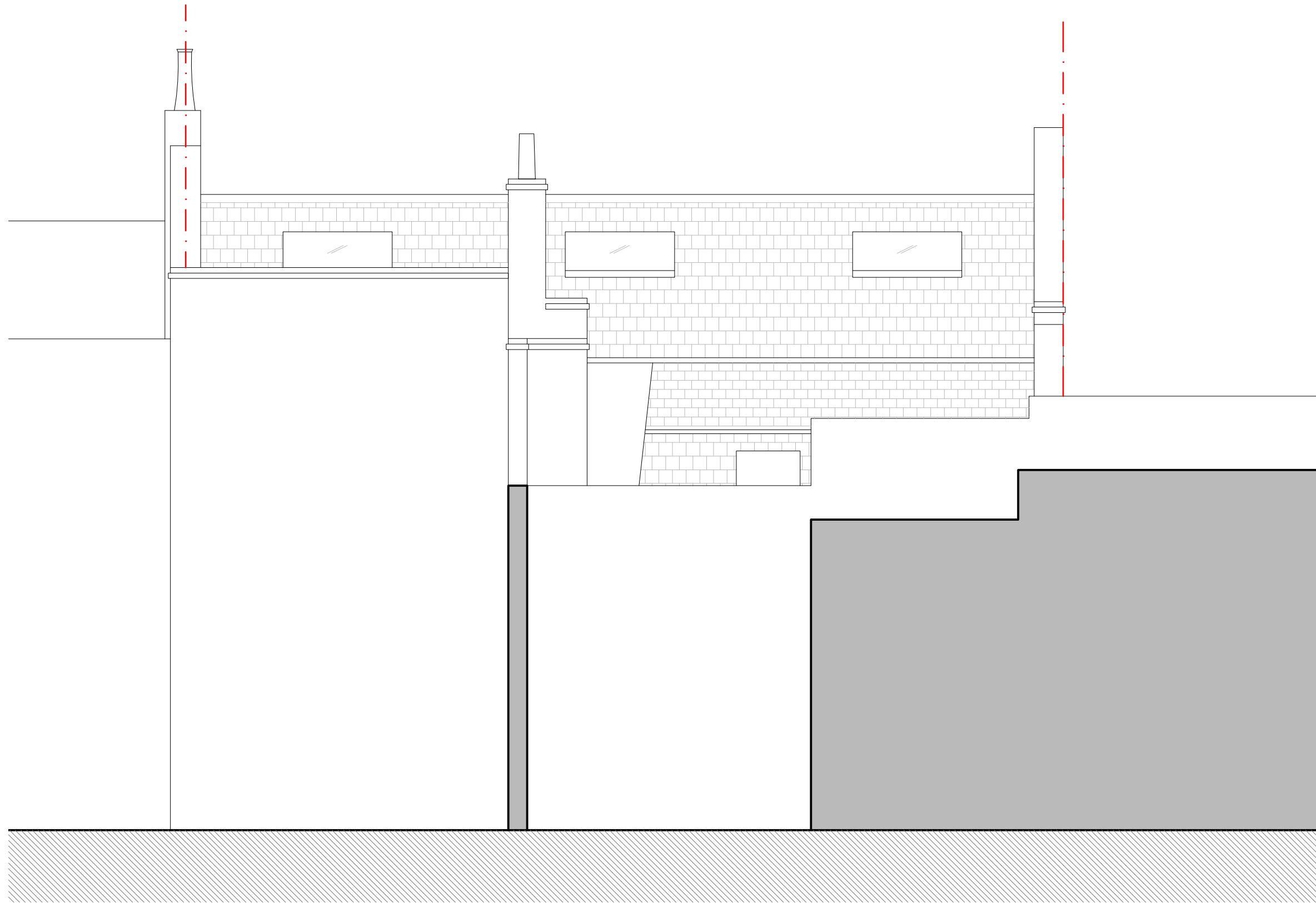
EAST ELEVATION
