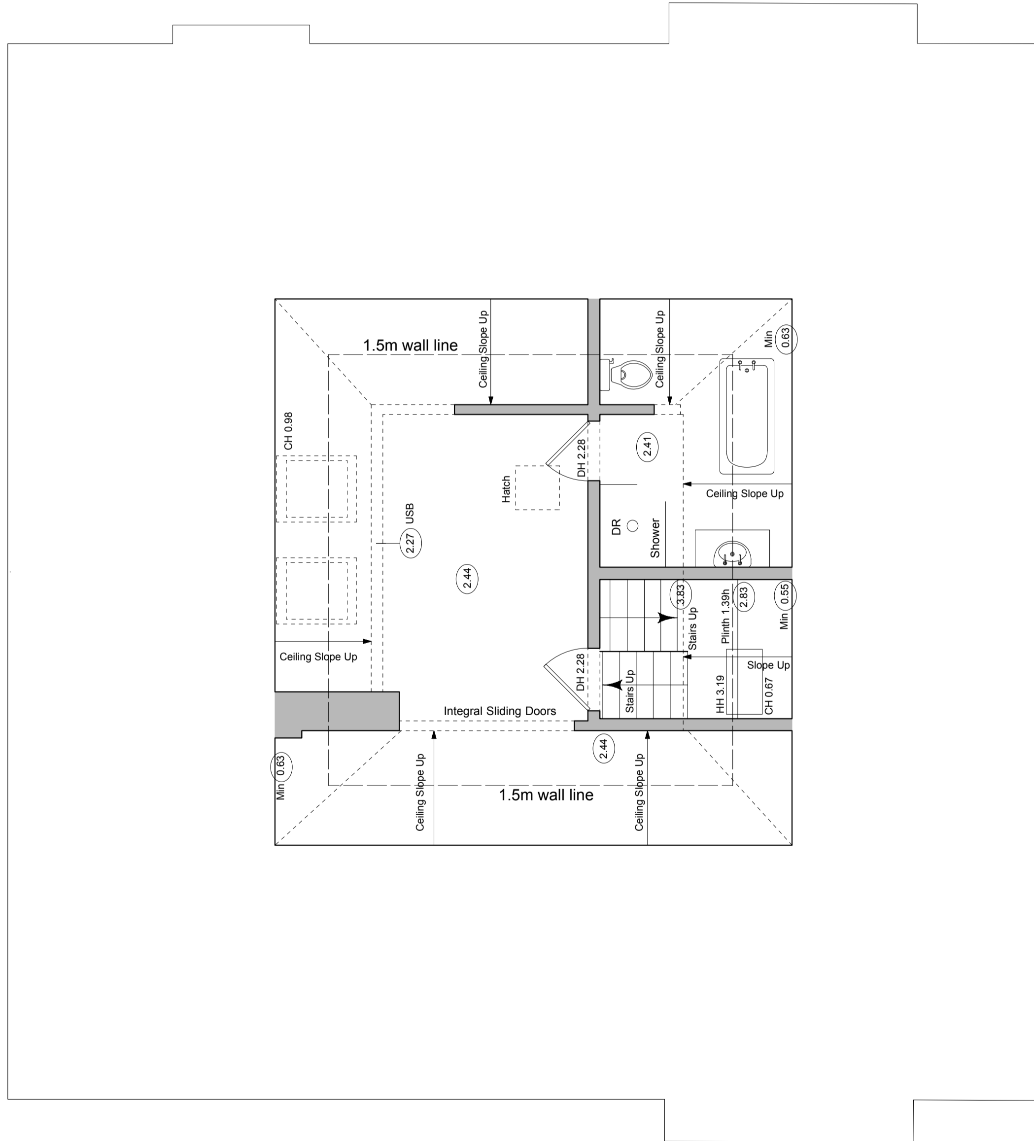
THIRD FLOOR
