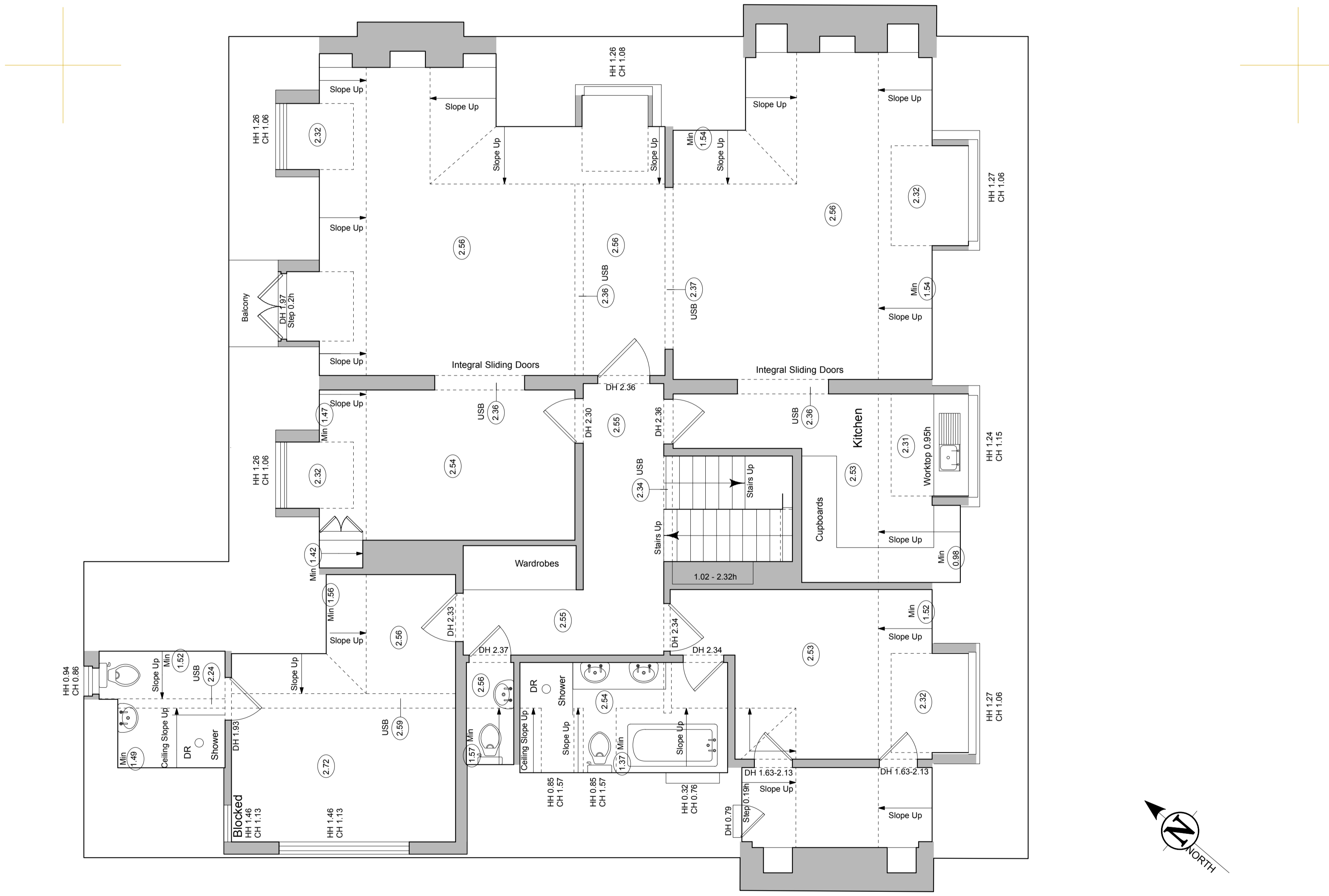
SECOND FLOOR
