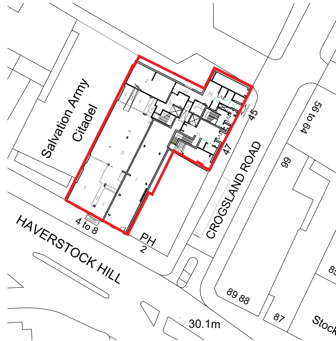
PROPOSED BLOCK PLAN 1:500 @ A3
