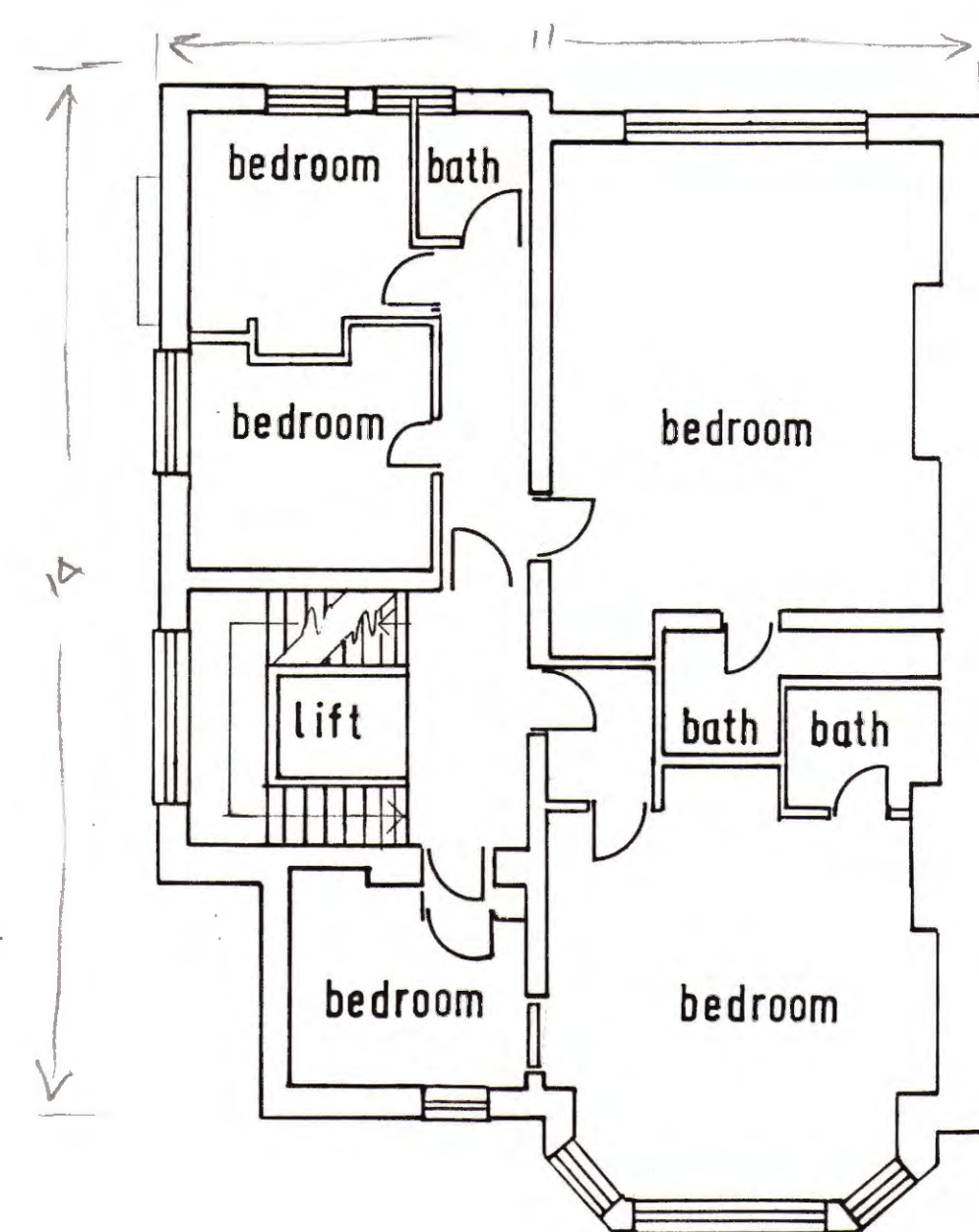
SECOND FLOOR
