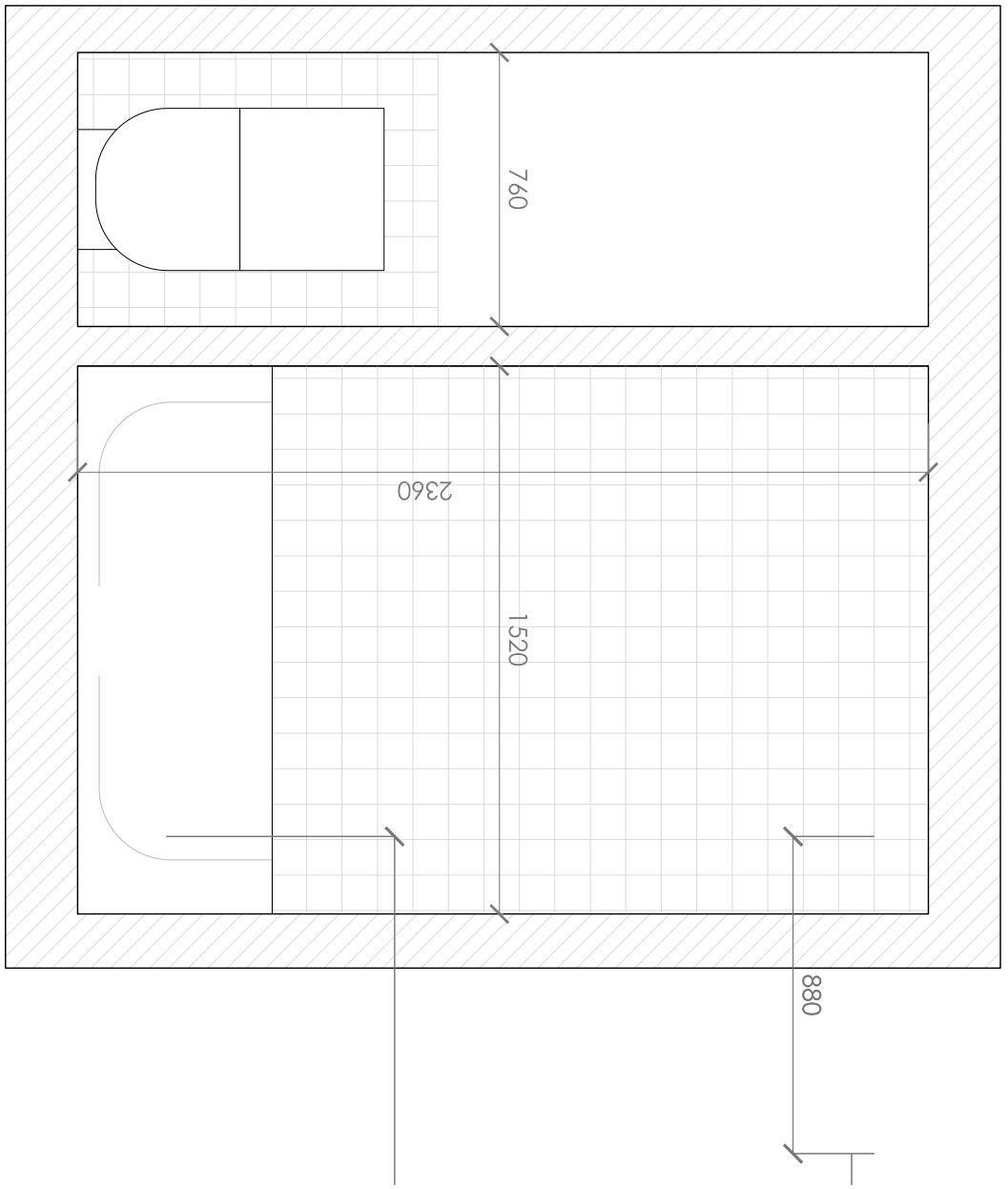
ELEVATION C
