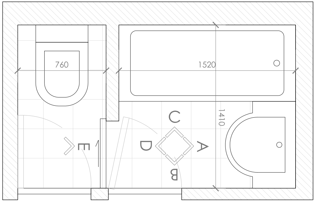
FLOOR PLAN
