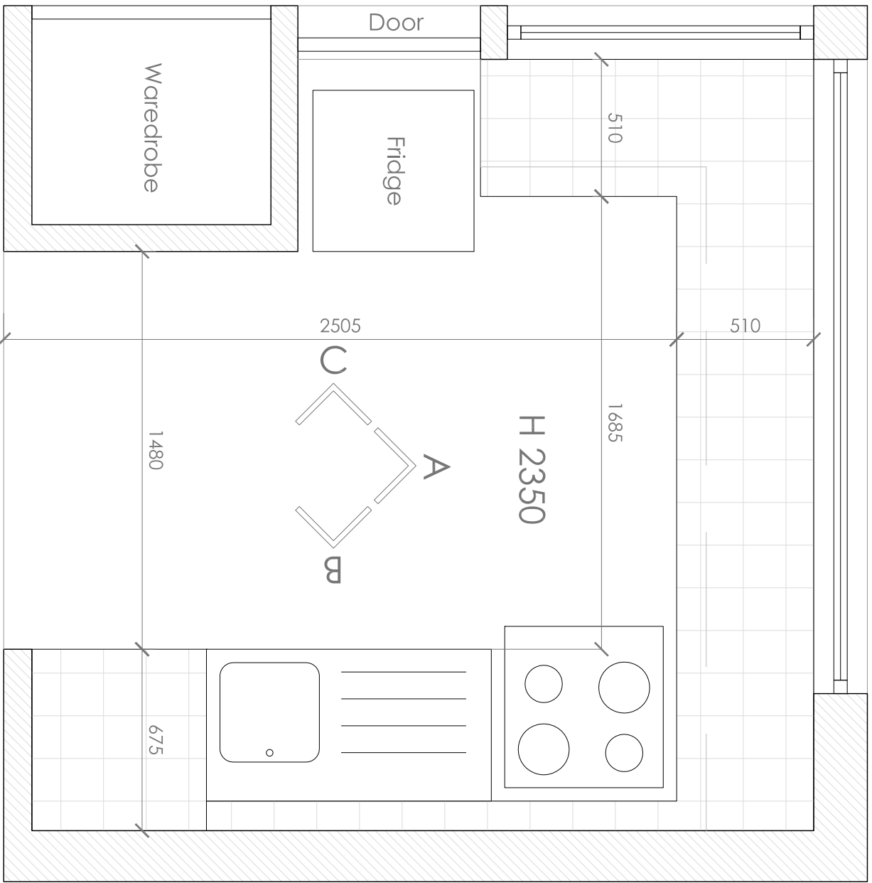
FLOOR PLAN
