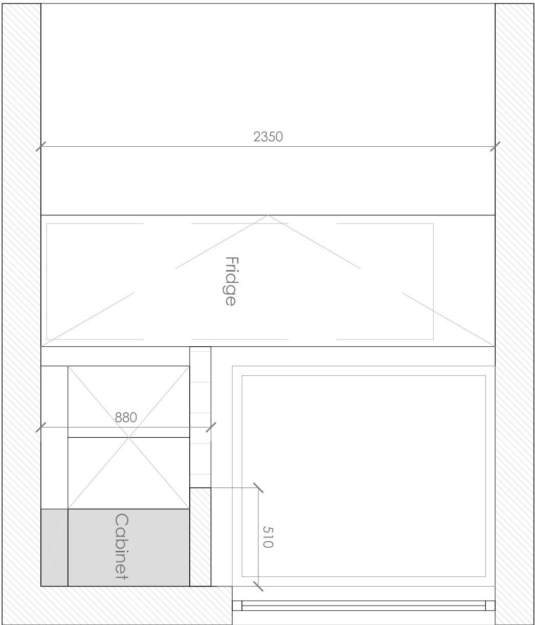
ELEVATION C
