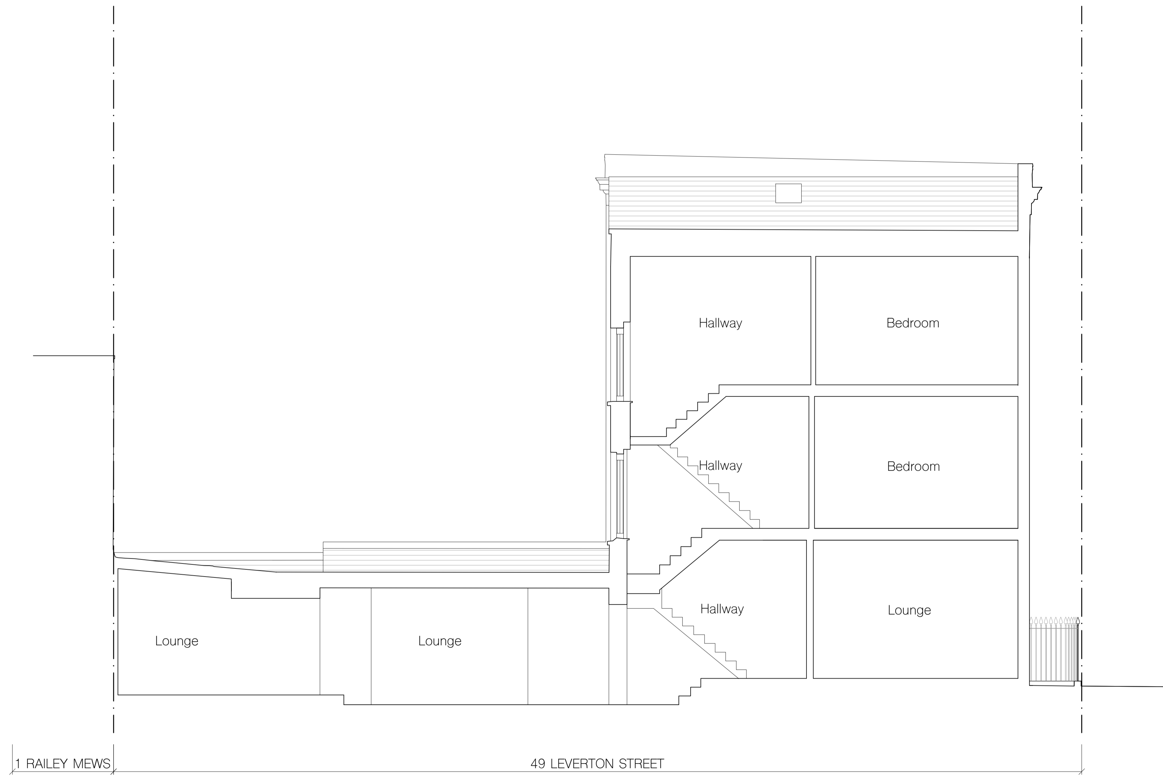
1 Existing section BB
