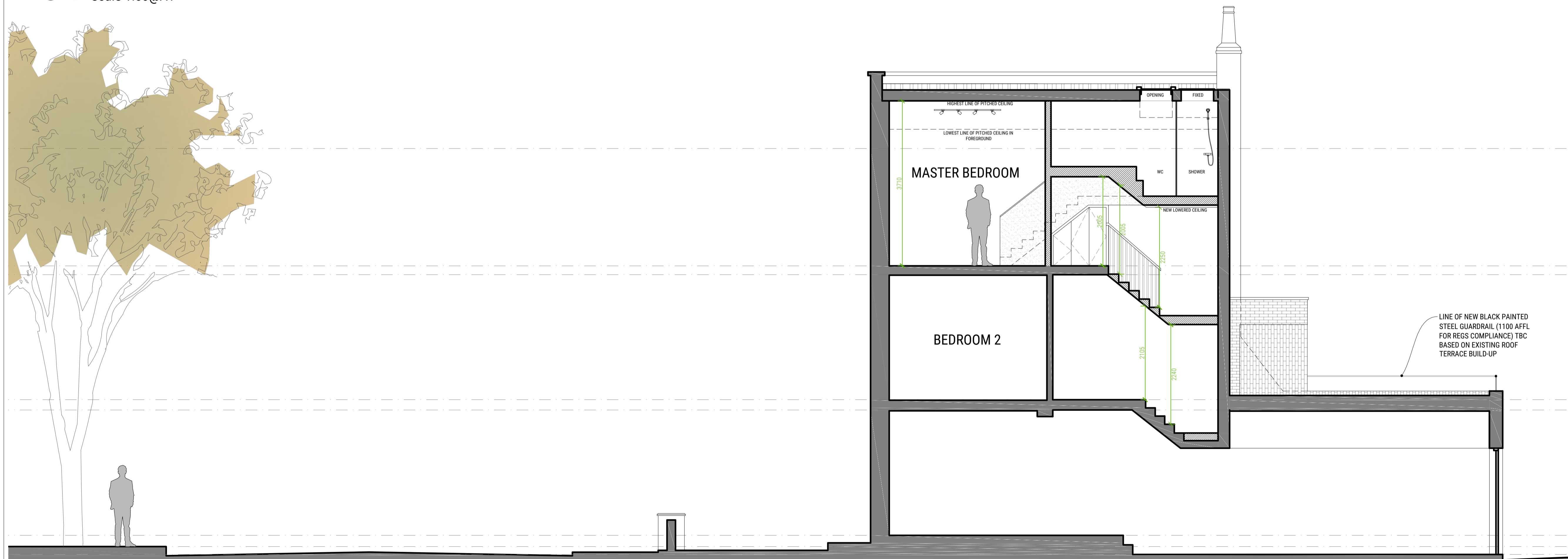
02 Proposed Long Section Scale 1:50@A1
