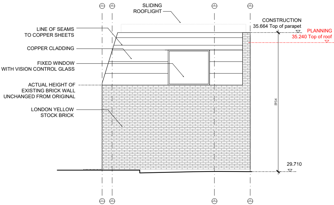
SOUTH ELEVATION - BUILT - 1:100@A3
