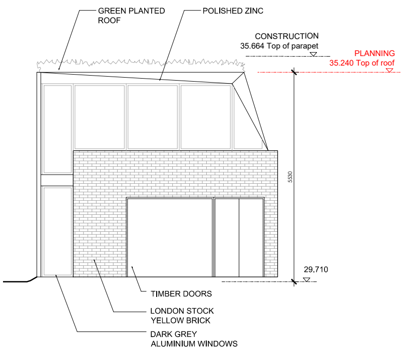
NORTH ELEVATION - PLANNING - 1:100@A3
