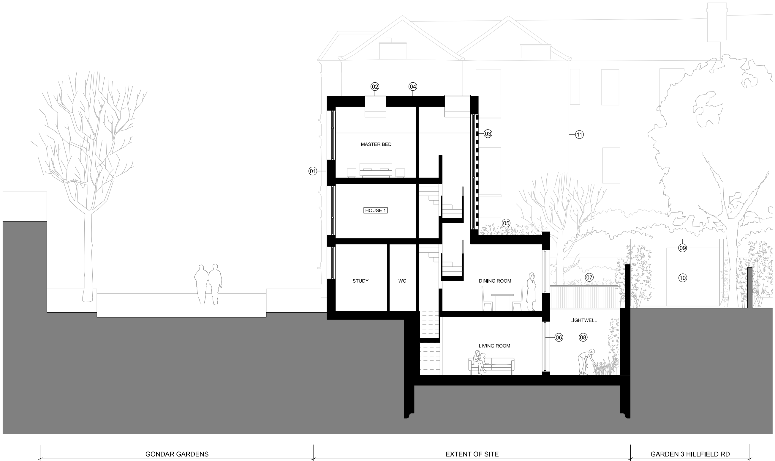
01 SHORT SECTION AA 1:100
