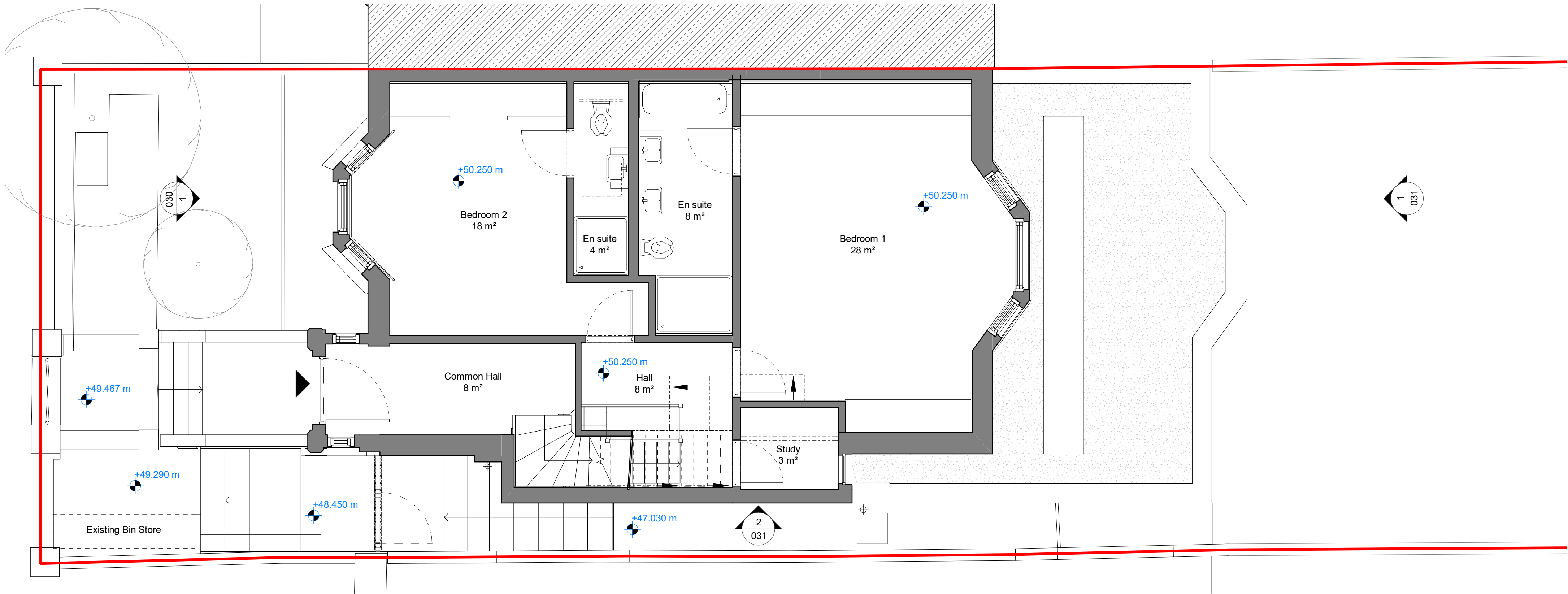
2 Existing Upper Ground Floor 1 : 50
