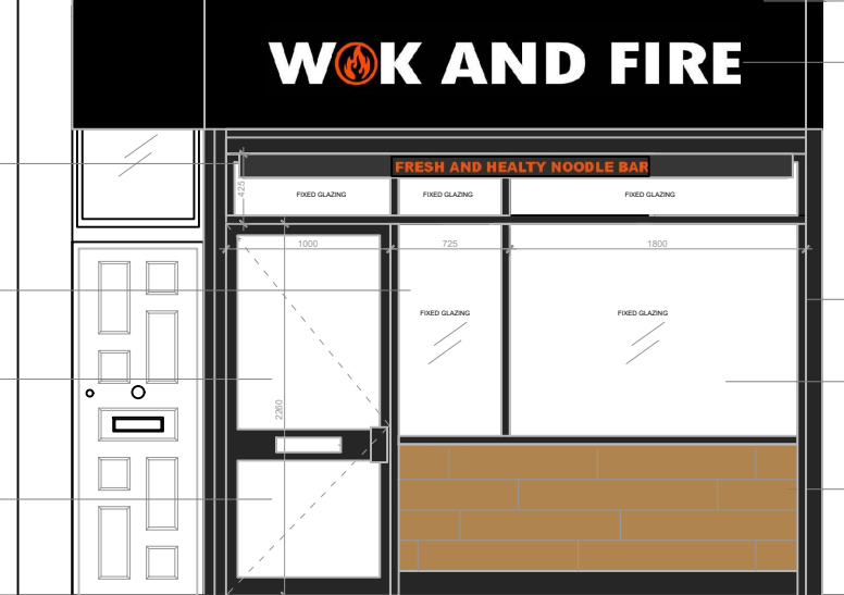
Proposed front elevation SCALE 1:50 @ A3
