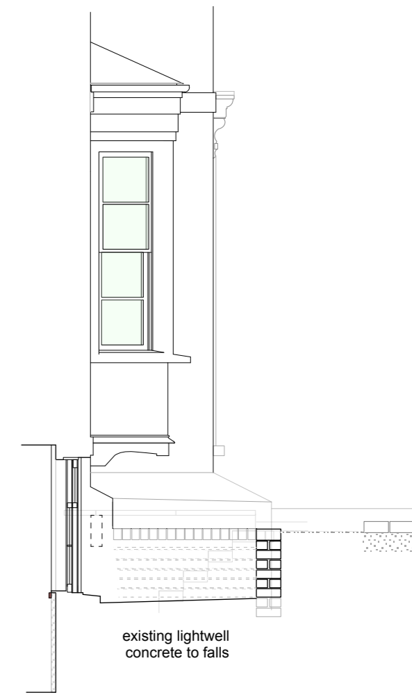
SECTION A 1:50
