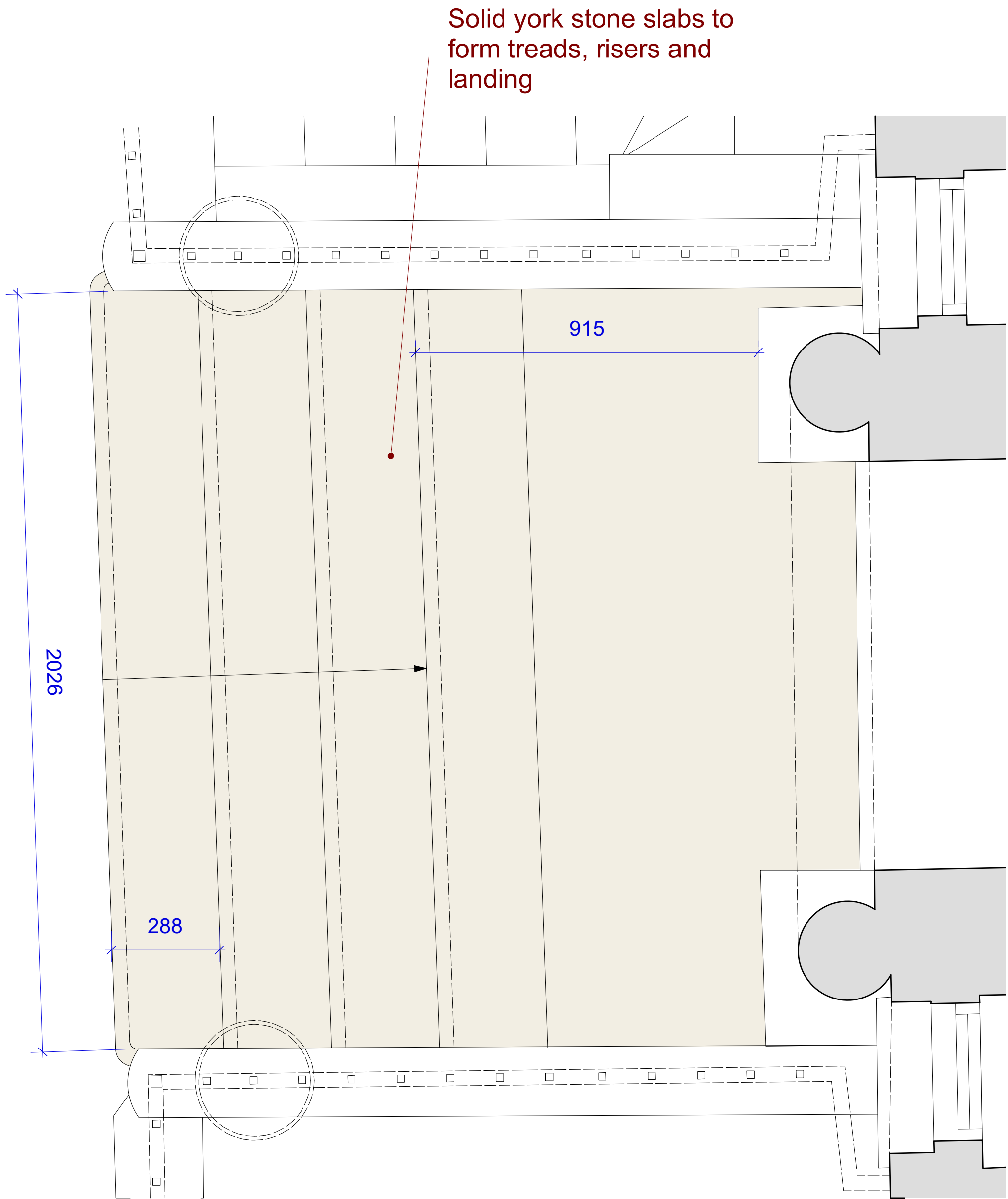
PLAN Scale 1:10
