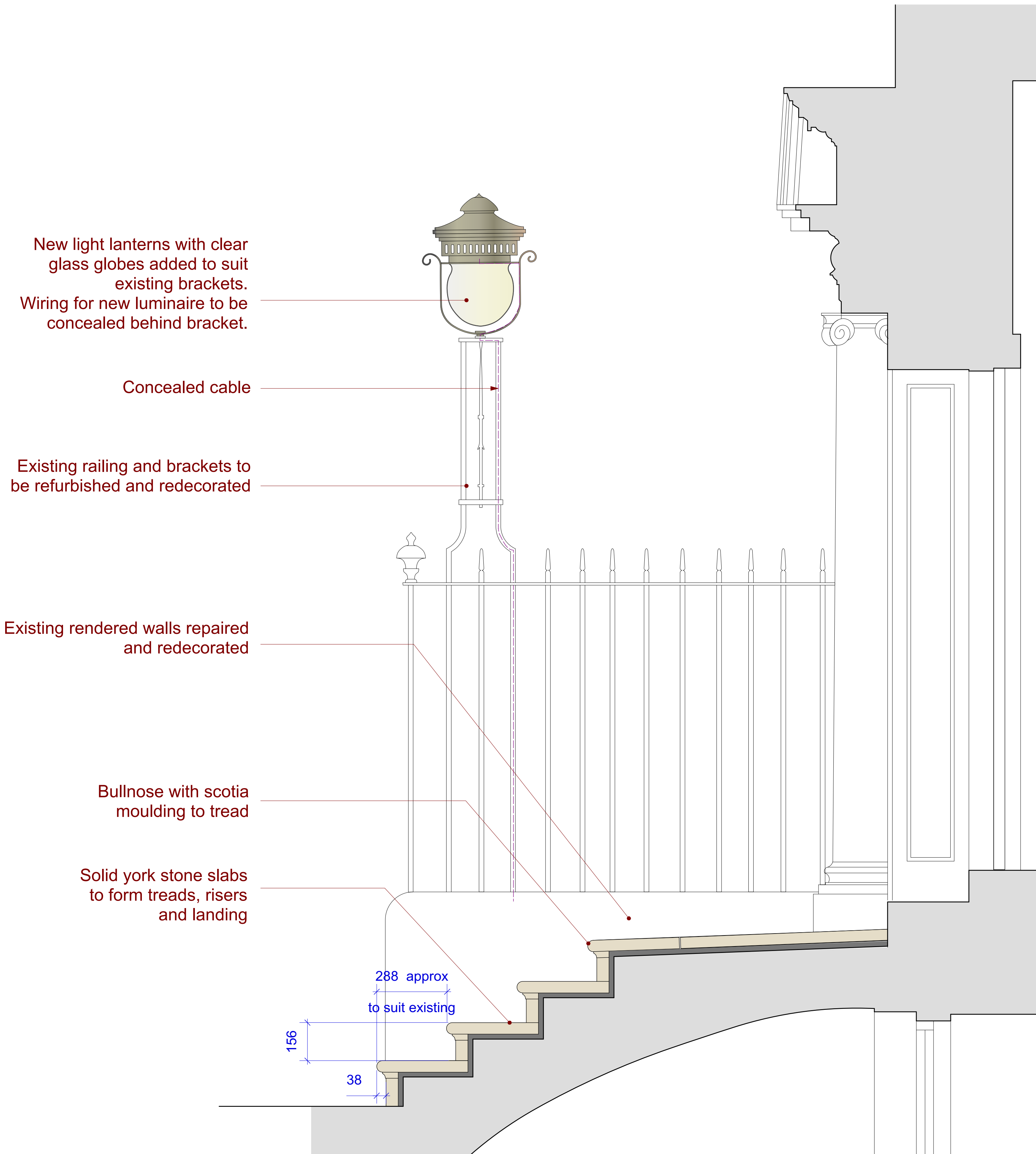
SECTION Scale 1:10
