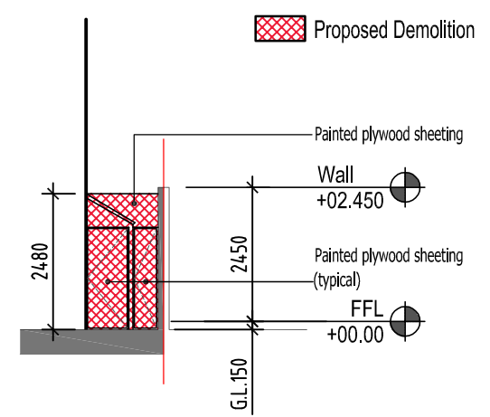
Existing Side Passage (Part) Front Elevation (West)
