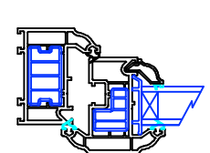
HORIZONTAL SECTION THROUGH OPENING CASEMENT AND FIXED PANEL TO SIDE
