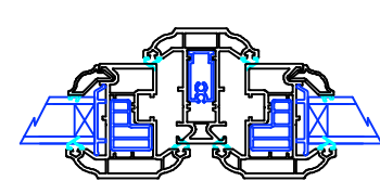
HORIZONTAL SECTION THROUGH TWO OPENING CASEMENTS SIDE BY SIDE
