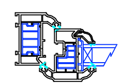
HORIZONTAL SECTION THROUGH TWO OPENING CASEMENTS SIDE BY SIDE
