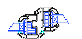
HORIZONTAL SECTION THROUGH OPENING CASEMENT AND FIXED PANEL TO SIDE
