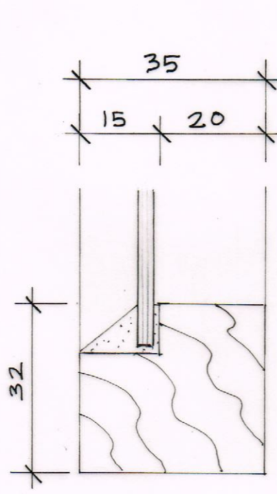
EXISTING GLAZING (CASEMENT) SCALE F/S
