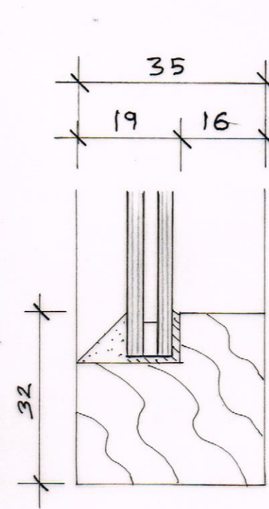
EXISTING GLAZING (CASEMENT) SCALE F/S
