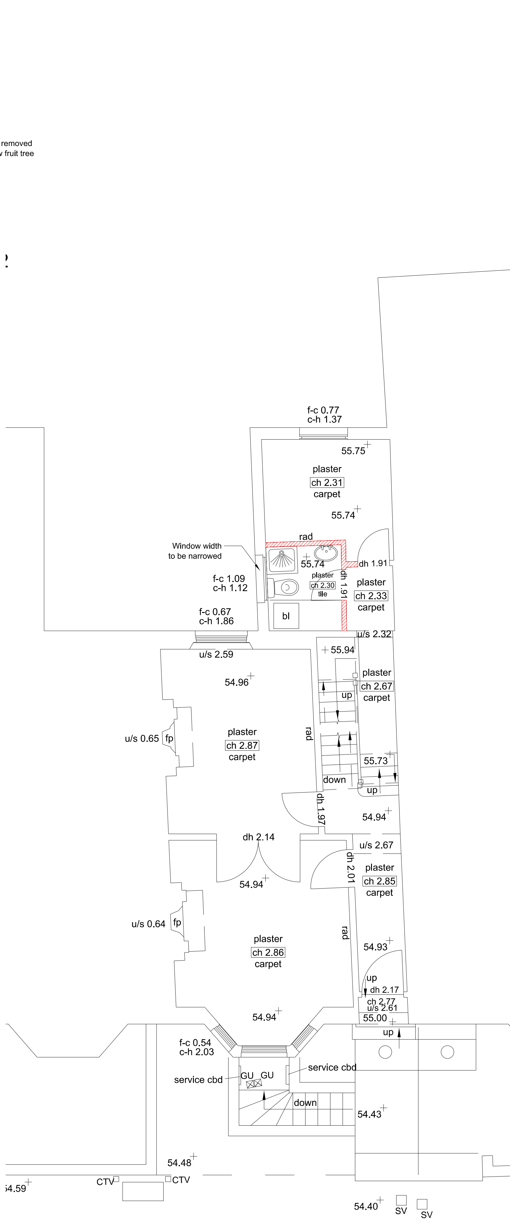
EXISTING UPPER GROUND FLOOR
