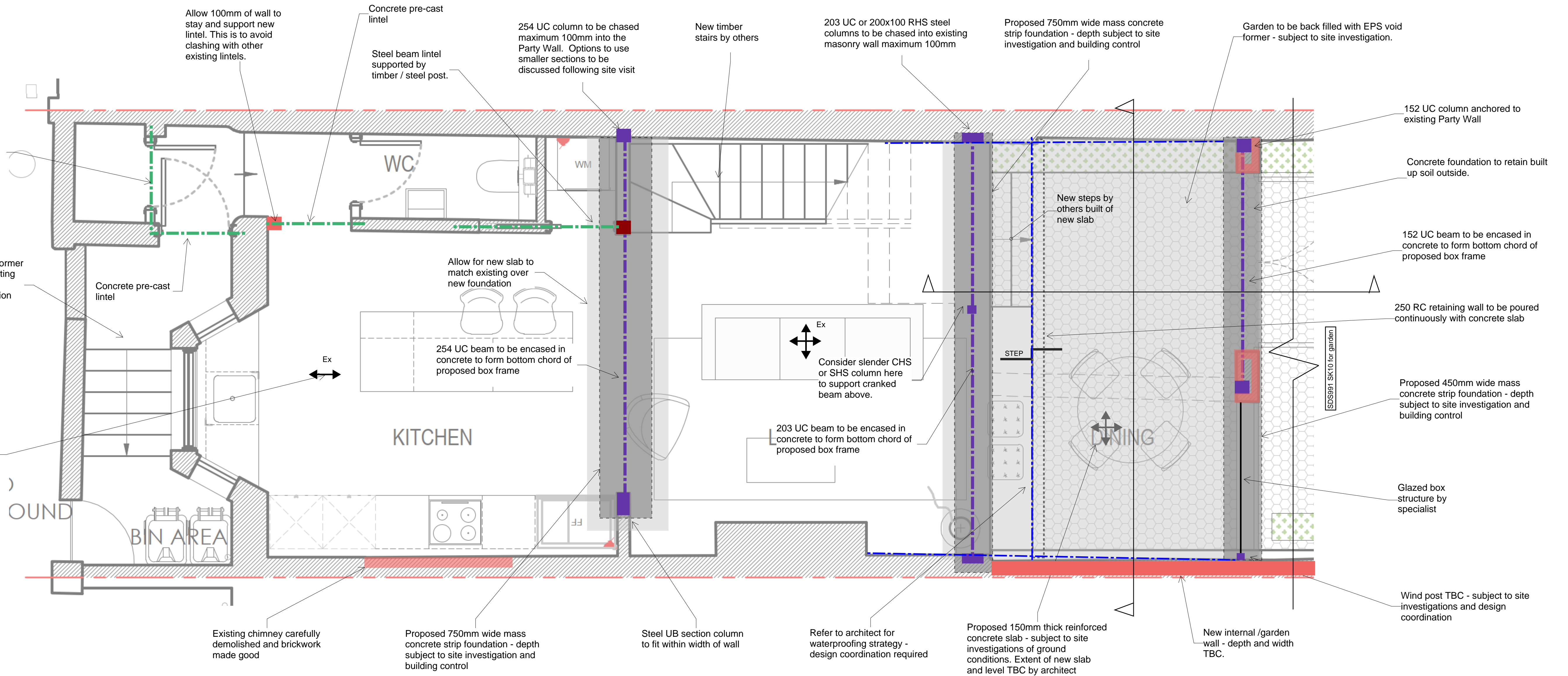
Lower Ground Floor Plan
