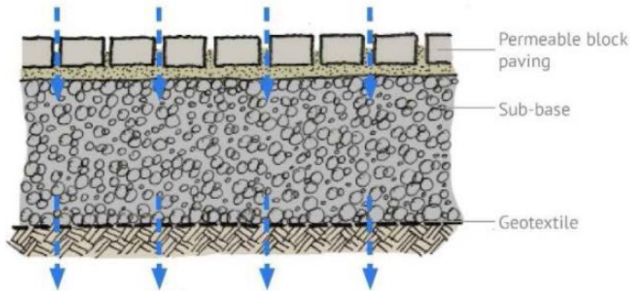
Figure 8: Typical section through permeable paving and sub-base showing infiltration
