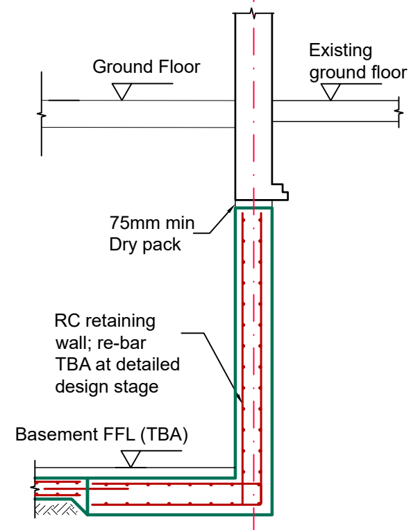
Section 2-2 Scale 1:50
