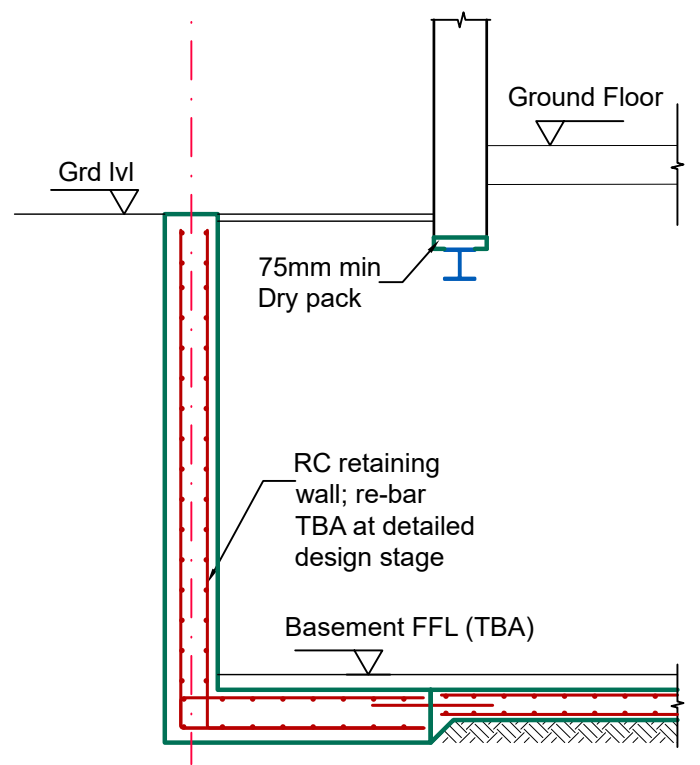
Section 1-1 Scale 1:50
