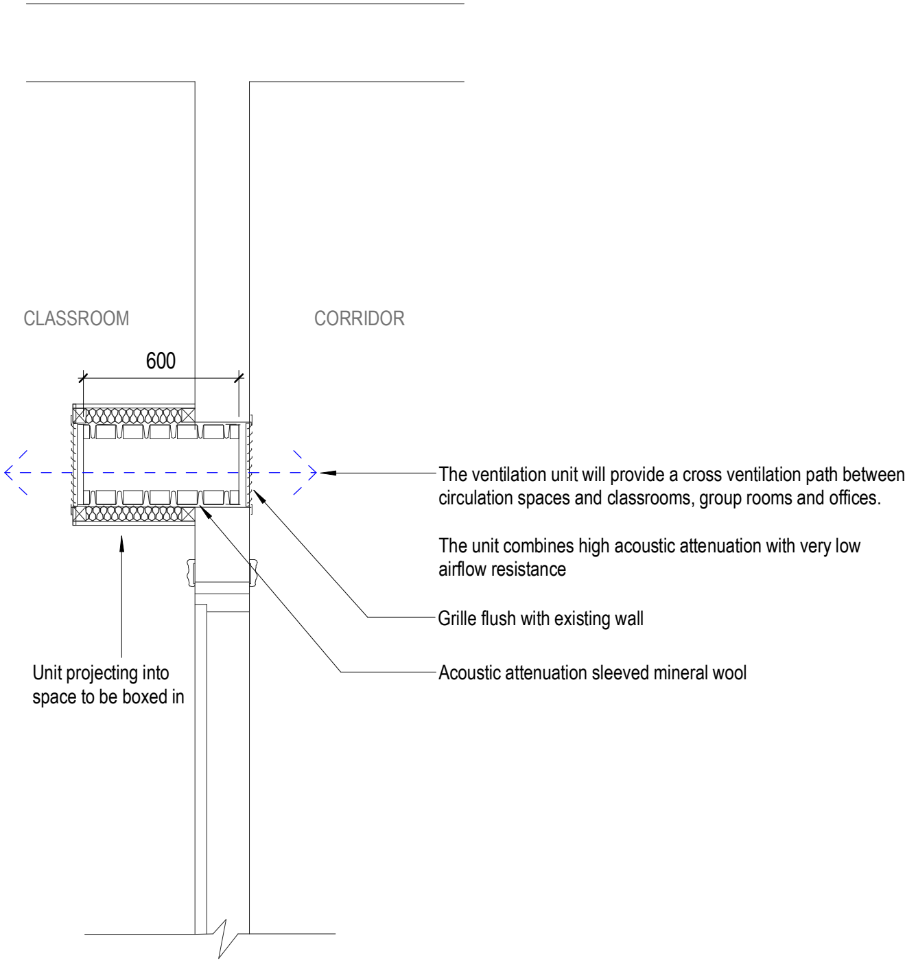
Setion through air ventilation unit
