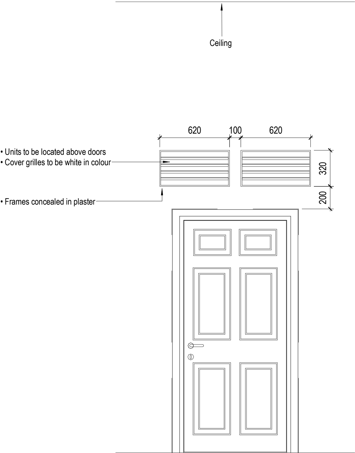
Elevation of classroom door with air ventilation unit above
