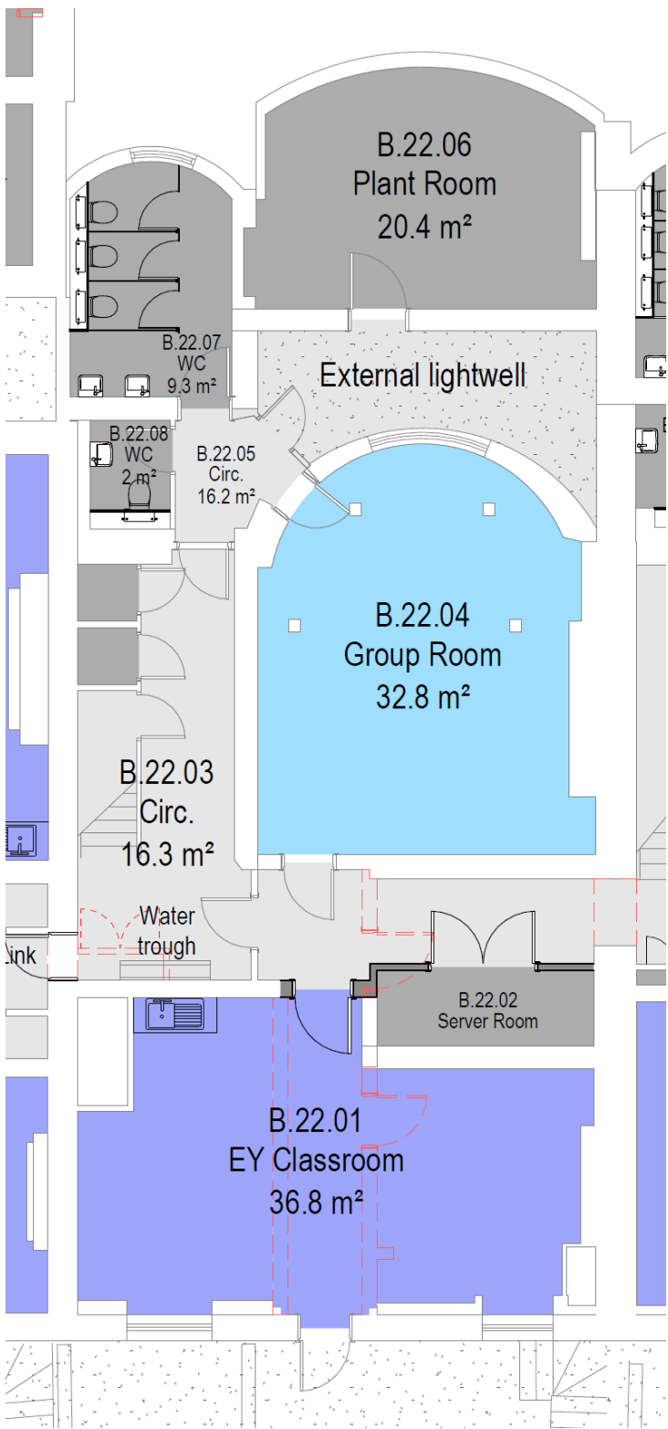
Proposed Lower Ground Floor Plan
