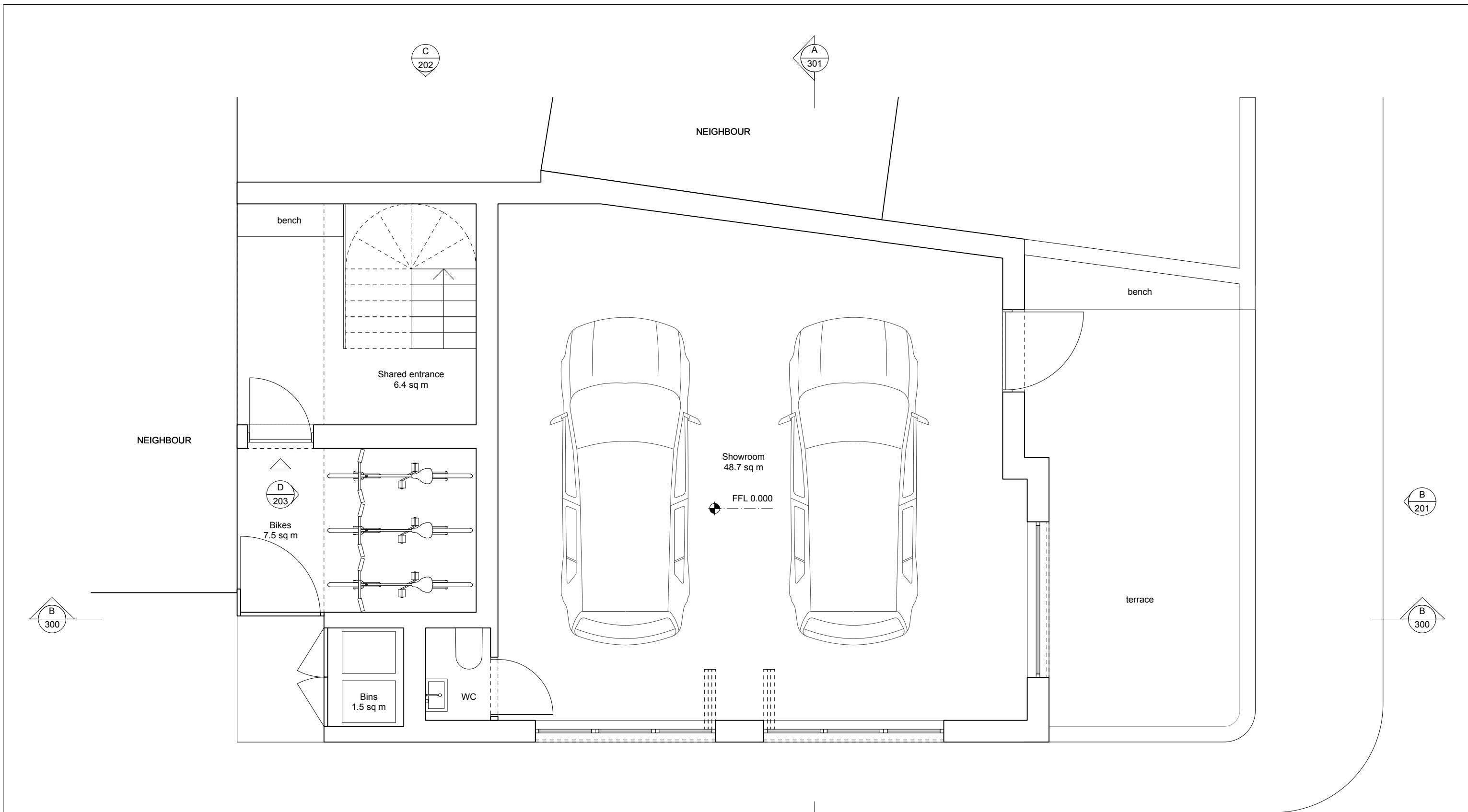
1 PROPOSED GROUND FLOOR PLAN 1:50@A3
