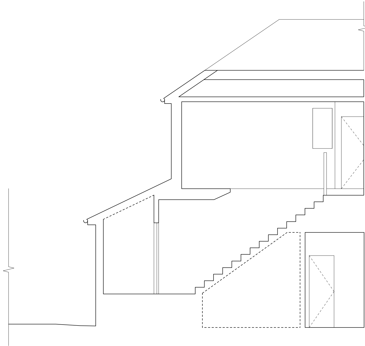
1 EXISTING SECTION A-A 1:50@A3
