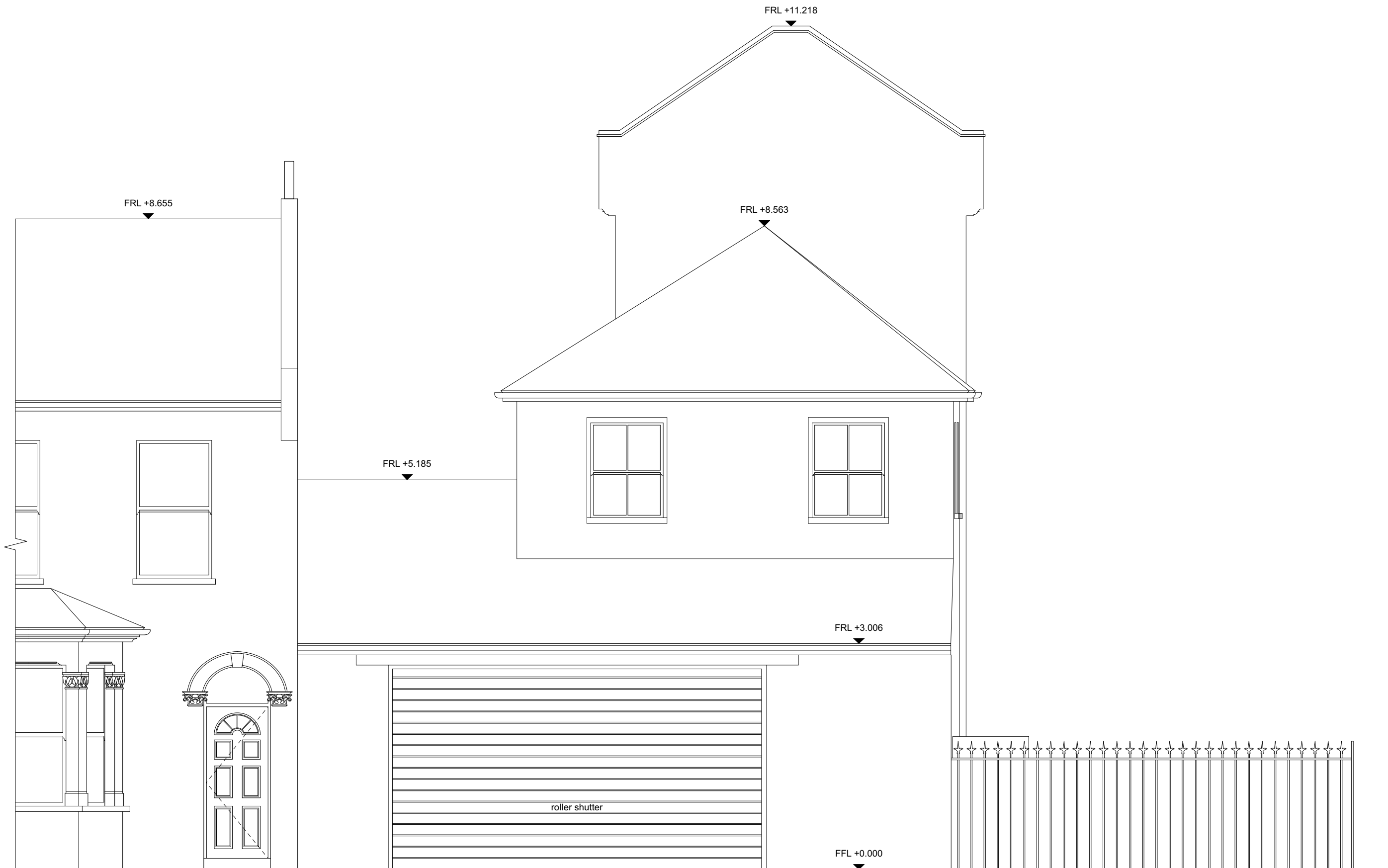
1 EXISTING FRONT ELEVATION 1:50@A3
