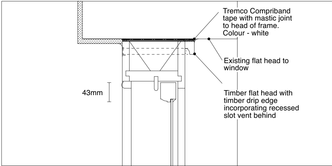
Head with flat head to lower ground & third floor
