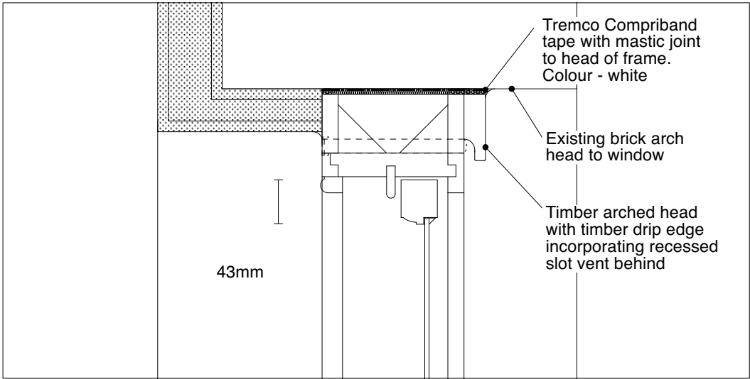
Head with brick arched head to rear brickwork
