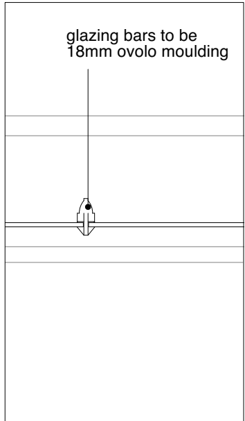
Vertical glazing bar (rear only)
