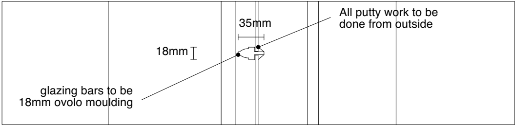
Horizontal glazing bar (rear façade only)
