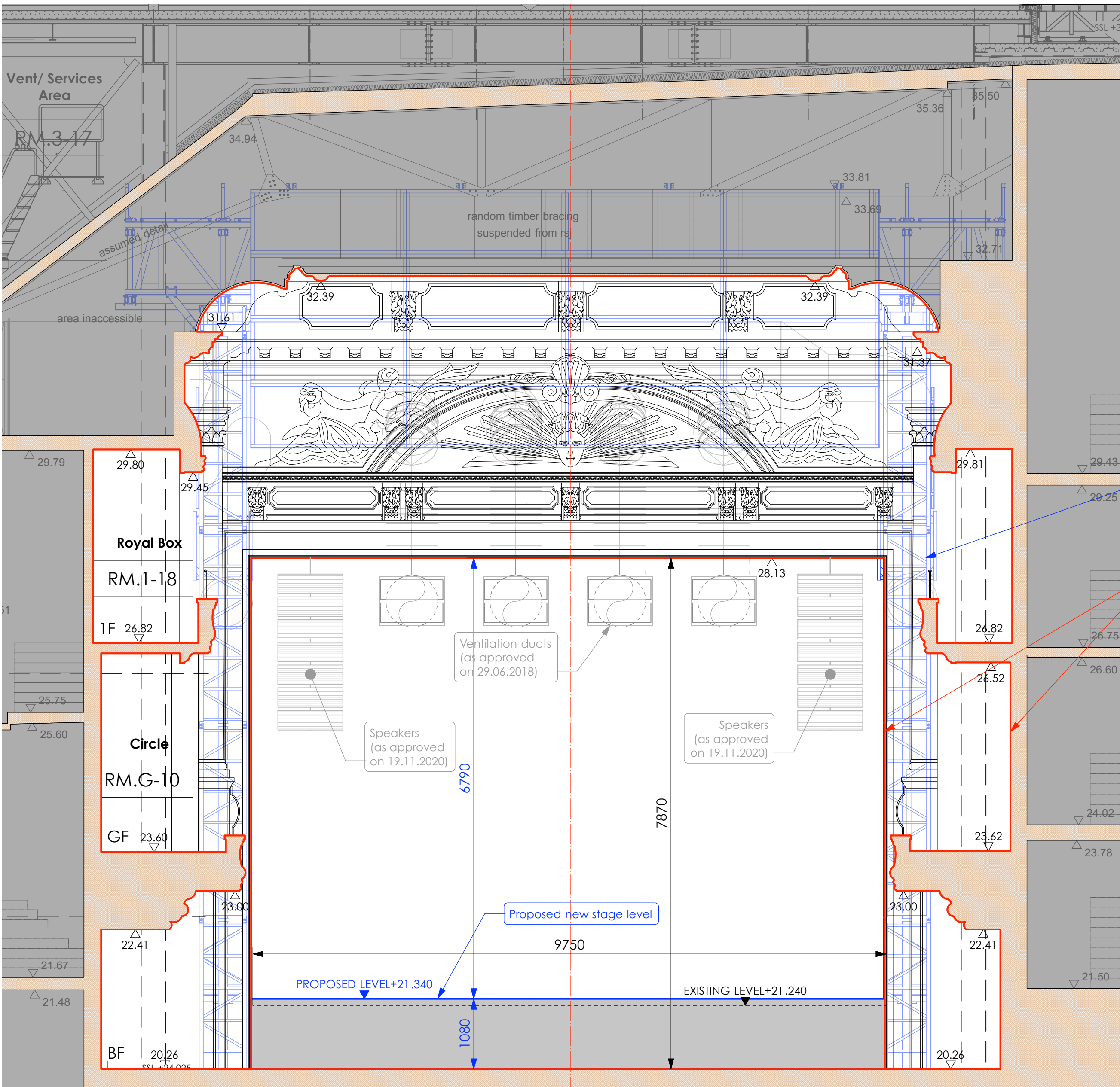
1 Flytower Rigging Elevation - view from Auditorium Scale: 1:50
