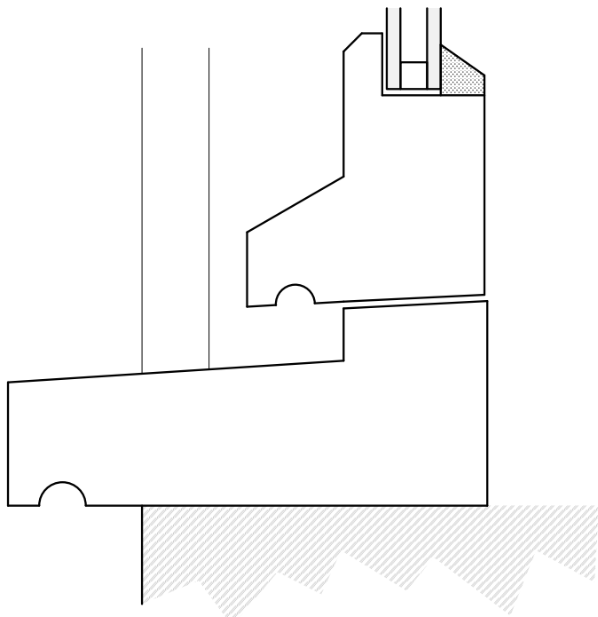
Existing Window - Door 1:2 @ A3
