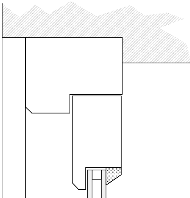
Existing Window - Door 1:2 @ A3
