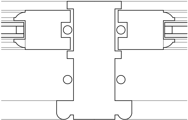
Existing Window - Jamb 1:2 @ A3
