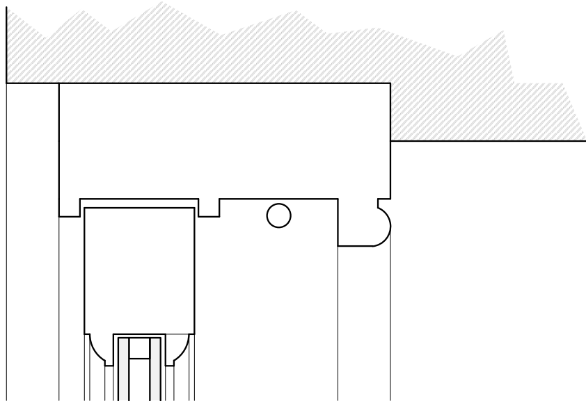
Existing Window - Head 1:2 @ A3
