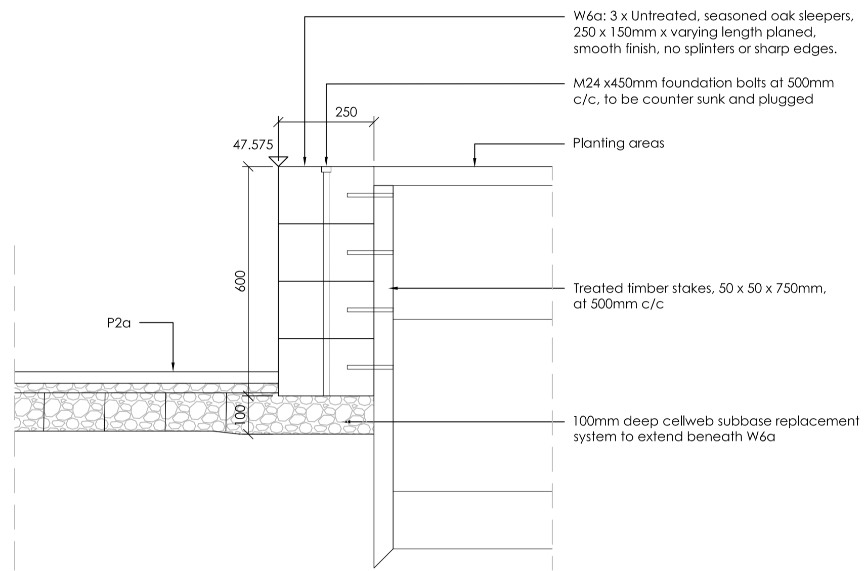
W6a Raised planter in no dig area Typical Detail Cross Section Q50/371A 1:10
